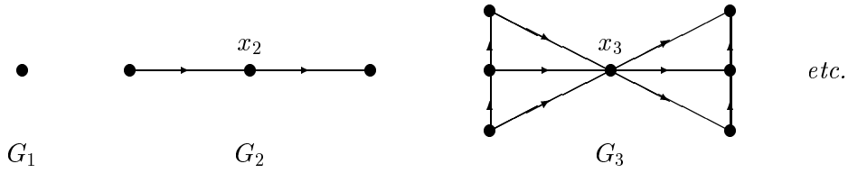
Figure 1: A sequence of oriented graphs G_i , i \geq 1 , with \vec{\chi}(G_i) = 2^i - 1
