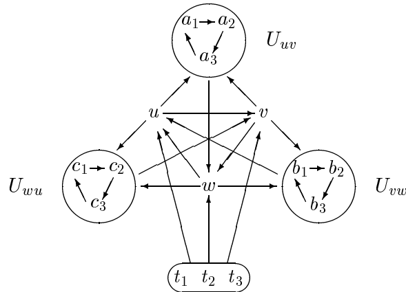
Figure 2: The structure of the graph U
