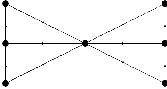
Figure 1: An oriented outerplanar graph with oriented chromatic number 7
