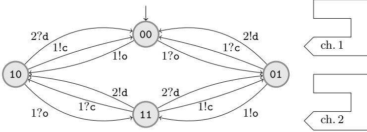
Fig. 3. Fifo System Representing the Connection/Disconnection Protocol
