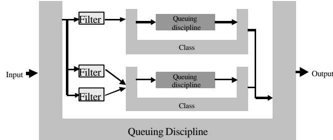
Fig. 3. Linux Traffic Control Components
