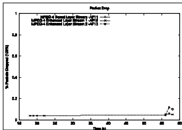
Fig. 13. Packet drops with IP Diffserv- Network Load >95% -
