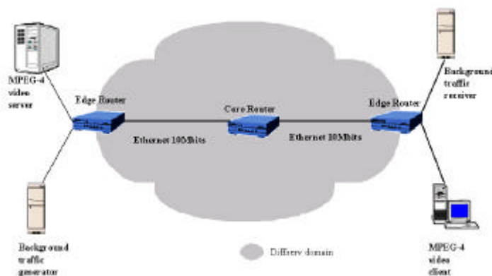
Fig. 5. IP DiffServ Network testbed
