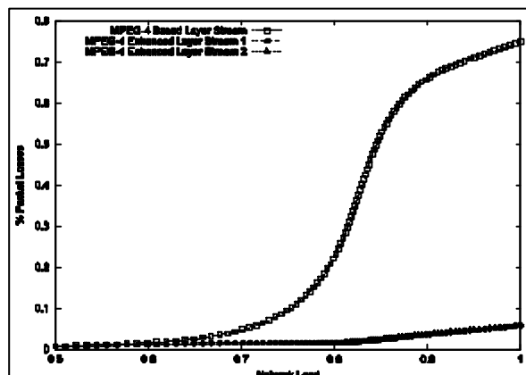
Fig. 8. MPEG-4 video packet Loss ratio vs Network load with IP Diffserv
