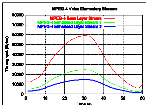
Fig. 7. MPEG-4 Video Layered Streams
