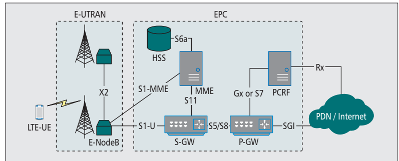
Figure 1. LTE network architecture.
