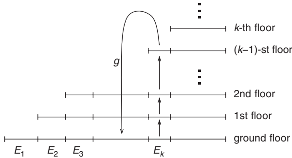
Figure 1.4. Kakutani–Rokhlin tower of g with time \rho
