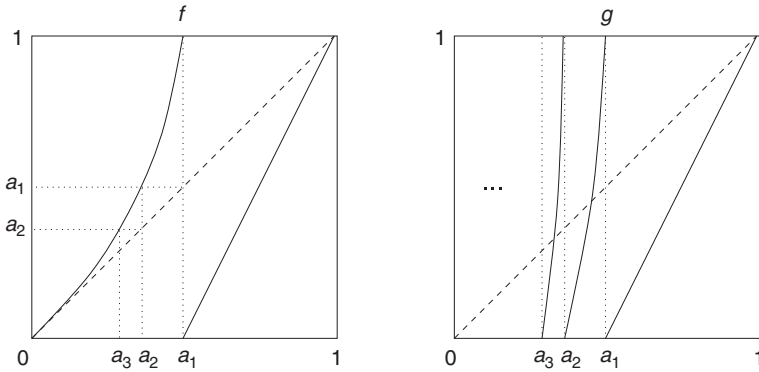
Figure 1.3. Construction of an induced transformation
