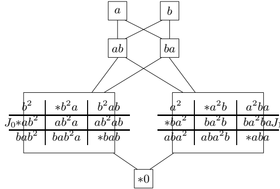
FIGURE 1. The semigroup S_1
