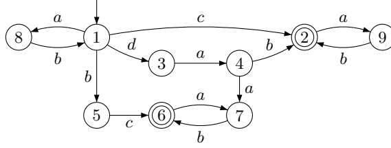
FIGURE 2. Automaton whose transition semigroup is S_2
