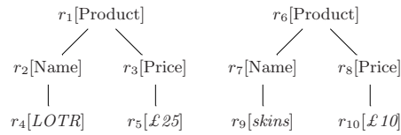
Fig. 3. Forest produced as the result of the TPQ \text{LQBill} \rightsquigarrow \text{RQBill} on document T .
