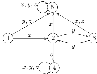
Figure 2: An automaton whose transition semigroup satisfies x^\omega y x^\omega z t^\omega = x^\omega y z t^\omega yet not in \mathbf{X}
