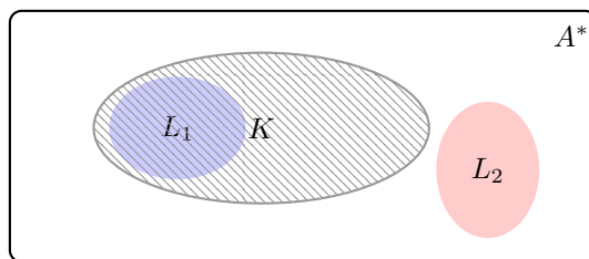
Fig. 2. K separates L_1 from L_2
