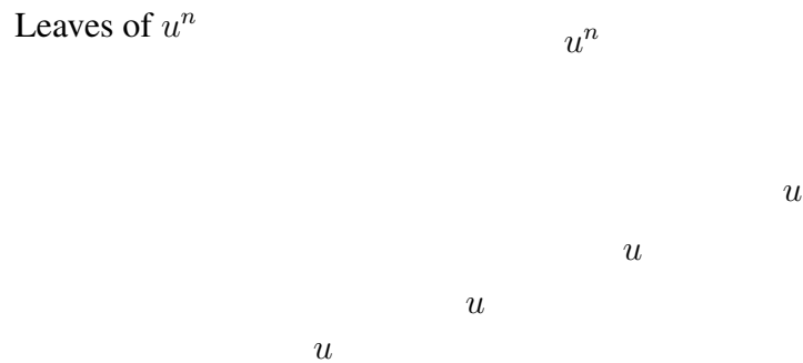
Fig. 2: The identity u^{n+1} = u \cdot u^n
