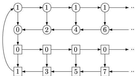
Fig. 1. Player 0's strategy must recall the highest odd vertex reached by player 1 in the lower row in order to answer with a higher even vertex in the second row.
