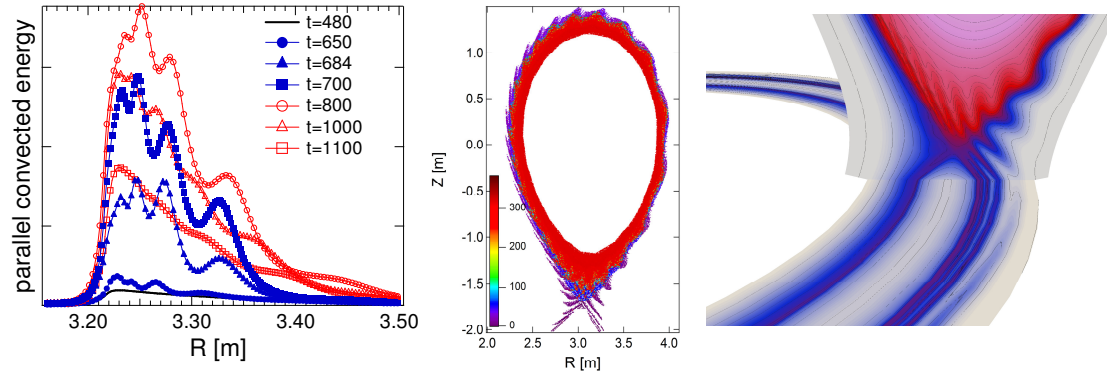
Figure 3.4 The parallel convected energy flux (in a.u.) to the outer target as a function of the major radius at the target for several time slices.
