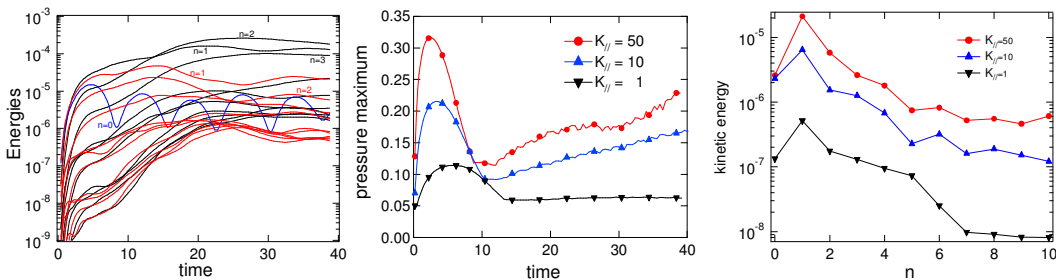
Figure 4.2a The evolution of the magnetic (black) and kinetic (red) energies for each toroidal harmonic as a function of time due to a ‘pellet’ perturbation at t=0 for \kappa_{||}=50 .
