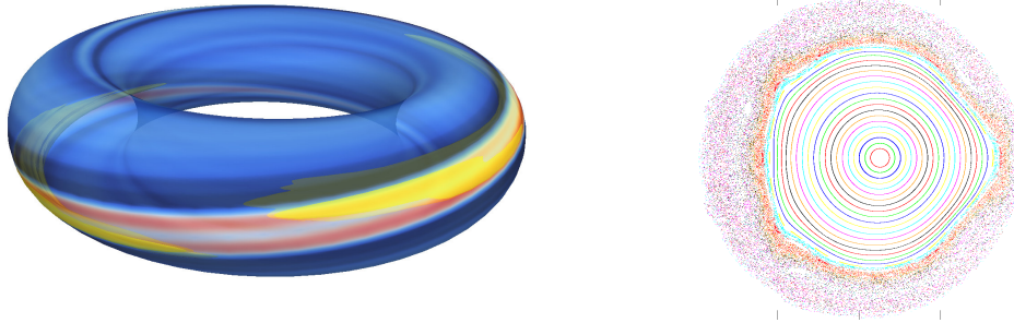
Figure 4.3a The temperature on a flux surface at t=26\tau_A showing a single helical ballooning type perturbation (colour scale from blue, T=6 \times 10^3 to red, T=8 \times 10^3 ). Also show (in yellow) is the density contour at twice the central density.
