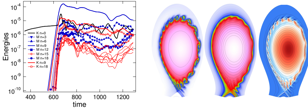
Figure 3.1 The magnetic ( M ) and kinetic energies ( K ) as a function of time for each toroidal harmonic.
