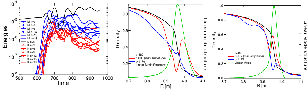
Figure 3.7 The time evolution of the magnetic ( M ) and kinetic energies ( K ) for each of the toroidal harmonics for a medium size ELM.
