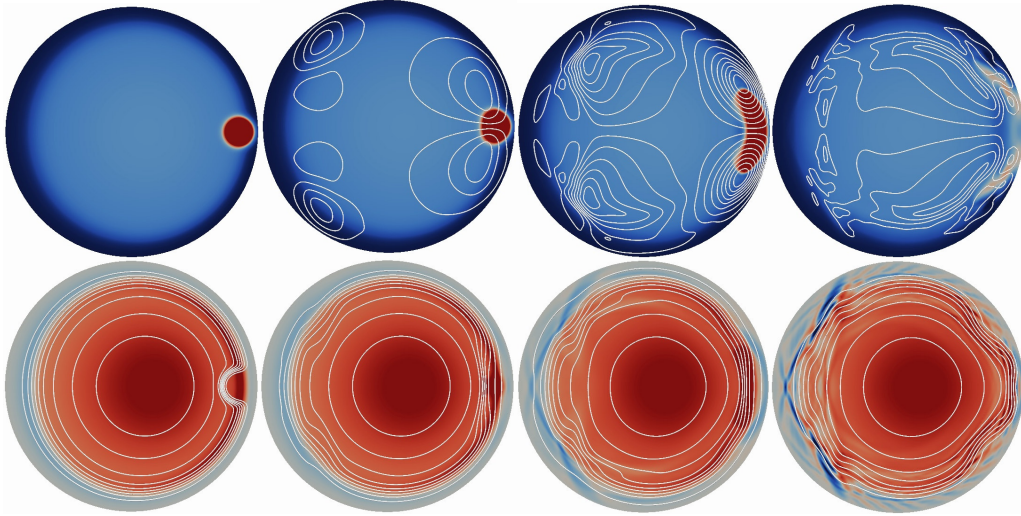
Figure 4.1 The evolution of the plasma density (top, color), the velocity flow lines (equi-potential lines) (top, contours), the current density (bottom, color) and temperature contours (bottom, contours) at t=0, 6, 10 and 26 \tau_A .
