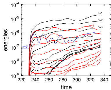
Figure 4.4 The evolution of the magnetic (black) and kinetic (red) energy for each toroidal harmonic ( n=0,10 ) Figure 4.5 The temperature on a flux surface just inside the separatrix ( 8 \times 10^4 < T < 2 \times 10^3 ) at t=330\tau_A . The density contour of twice the central density is shown in yellow. The initial density perturbation was injected in the pedestal on the left hand side (in the figure).
