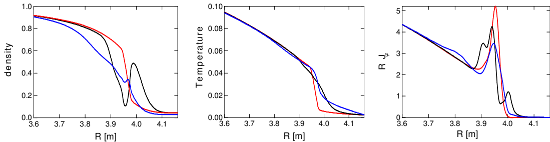
Figure 3.3 Density and temperature and toroidal current density in the outboard mid-plane at t=480 \tau_A , t=700 \tau_A and t=1170 \tau_A .
