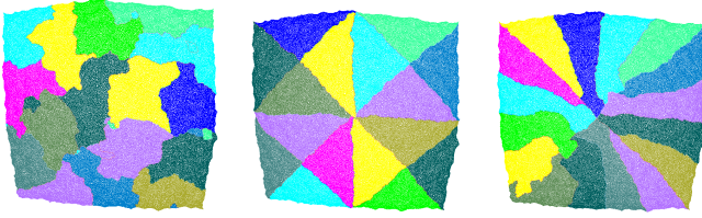
Figure 6. Partitioning of the graph of matrix darcy003 in 16 domains with SCOTCH. From left to right, the method applied was greedy graph growing, double greedy graph growing and halo-first greedy graph growing.
