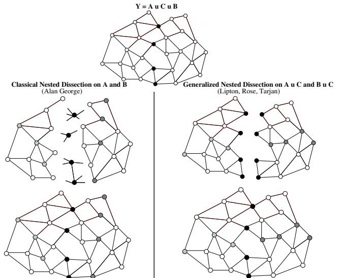
Figure 1. On the left : classical recursion which is performed on P_0 and P_1 . Objectives are to balance the sizes of the subgraphs and to minimize the separator size. However, halo sizes, represented by the nodes in black and grey, can be unbalanced: they are respectively 4, 5, 6 and 8. On the right : recursion is performed here on P_0 \cup S and P_1 \cup S and the halo vertices are balanced among the parts, leading to interface sizes equal to 5, 5, 6 and 6.
