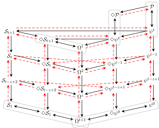
Fig. 1 Grid of failure detector classes
