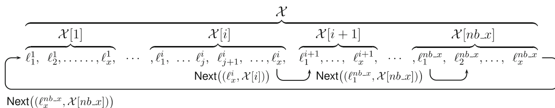
Fig. 6 The Next() function on the logical ring (\ell, X)
