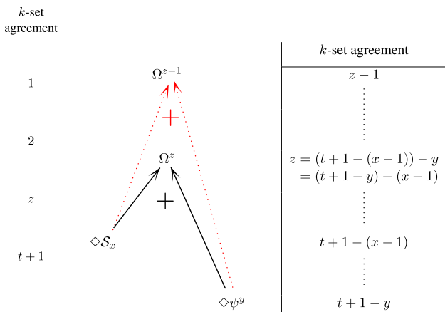
Fig. 2 Additivity of \diamond S_x and \diamond \psi^y
