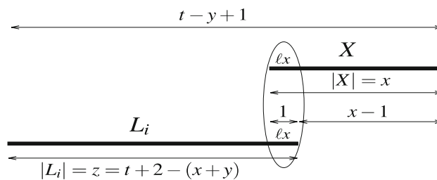
Fig. 9 When the upper wheel stops looking for a new L_i set
