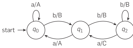
Figure 1. A simple Mealy machine.
