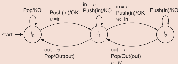
Figure 10. A register automaton.
