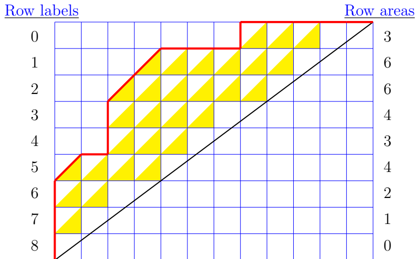
FIGURE 1. The (12, 9) -Schröder path 0000\bar{2}22\bar{3}7\bar{7} .
