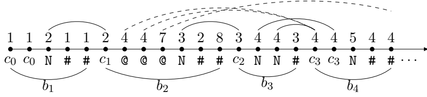
Fig. 3.7: LTL^\downarrow(F) cannot avoid having repeated consecutive symbols.
