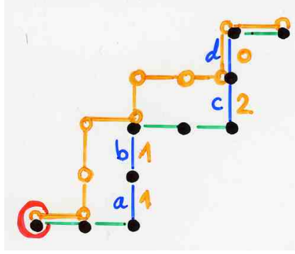
FIGURE 16. (with Figure 15 (left)) Lemma 7.
