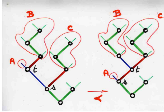
FIGURE 22. (with Figure 8) The covering relation in \text{Tam}(v) and the corresponding rotation in \overleftarrow{T} (ordinary Tamari with complete binary trees).
