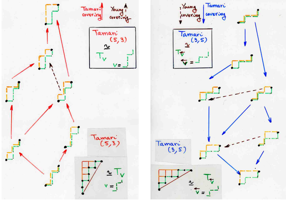
FIGURE 9. Duality and rational Catalan combinatorics: The lattices \text{Tam}(5,3) and \text{Tam}(3,5) .
