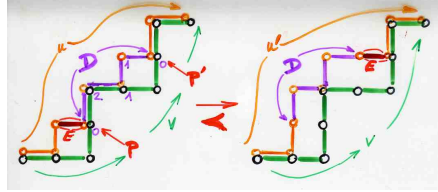
FIGURE 8. The covering relation defining the poset \text{Tam}(v) .
