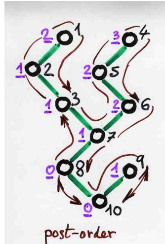
FIGURE 21. (with Figure 7) Lemma 12.
