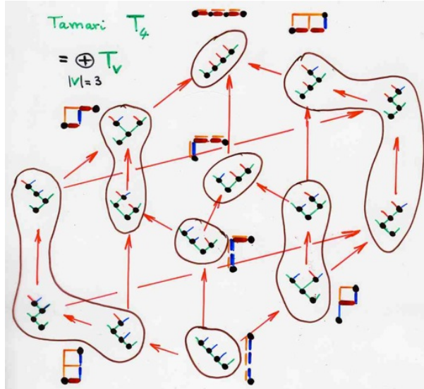
FIGURE 10. The decomposition of the Tamari lattice on complete binary trees with 4 interior vertices into the union of 8 disjoint intervals \text{Tam}(v) (Theorem 3).
