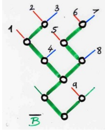
FIGURE 14. Second definition of the canopy.
