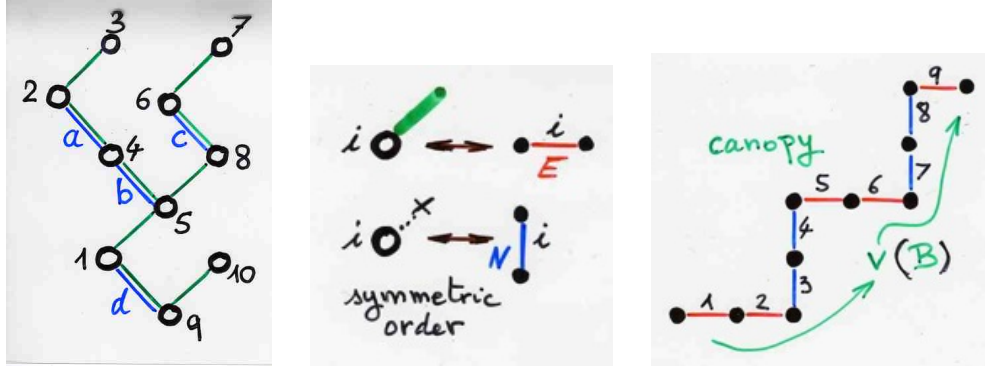
FIGURE 15. Third definition of the canopy (left and middle). The canopy (right).
