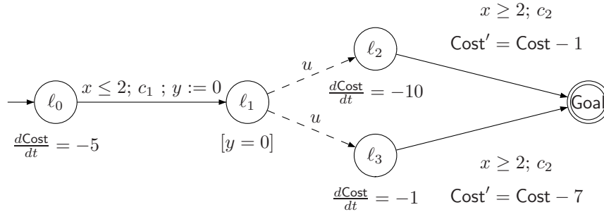
Fig. 4. The Linear Hybrid Game Automaton \mathcal{H} .
