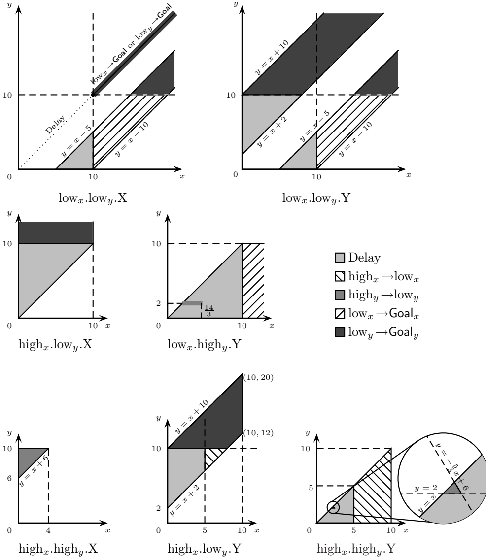
Fig. 9. Optimal Strategy for the Mobile Phone Example
