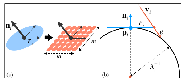
Figure 4: (a) Illustration of the upsampling algorithm. (b) 2D view to illustrate our view dependent geometric error. The tangent disk representing \mathbf{p}_i is displayed in blue and the viewing ray in red.
