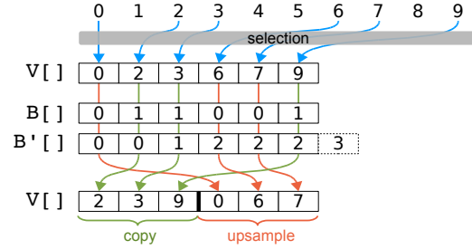
Figure 8: Illustration of the prefix sum based classification used in our low level temporal coherence algorithm.
