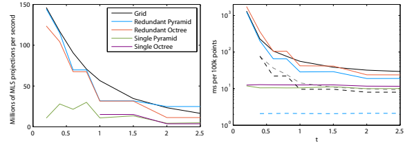
Figure 11: Performance of the MLS projections (left) and construction time (right) for varying values tradeoff t and for different data structures. The solid and dashed lines stand for the CPU and GPU DS constructions respectively.
