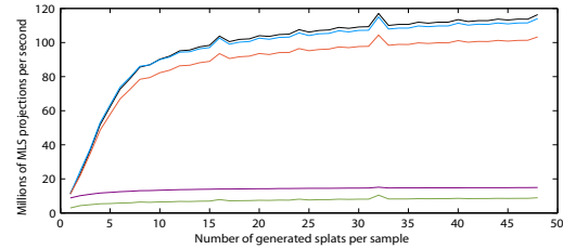
Figure 12: Performance of the MLS projection (in million of projection per second) according to the number of generated splats per sample. We use the same color scheme than in figure 11.
