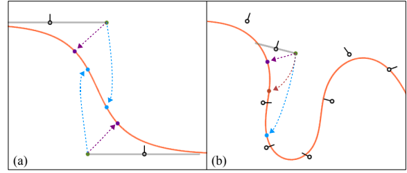
Figure 6: Comparisons of the three projection procedures for some splat extremities. Blue: simple. Red: almost orthogonal. Magenta: orthogonal. Note that in (a) the simple and almost orthogonal operators overlap.
