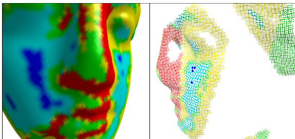
Figure 5: Illustration of our view dependent geometric error metric with color coded density. The right picture shows the generated splats utilized for rendering the left images. Note the accurate culling (view and backface) and the higher density near the silhouettes.
