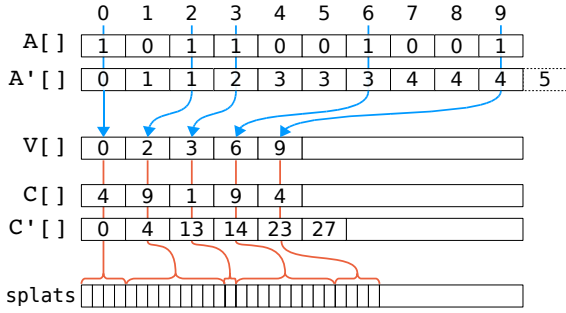
Figure 7: Parallel implementation of the selection (blue part) and upsampling (red part) algorithms.
