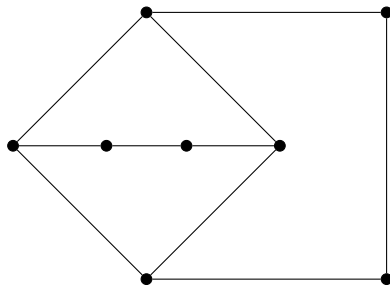
Figure 7: A graph G with mad(G) = \frac{5}{2} and \chi'_s(G) > 7
