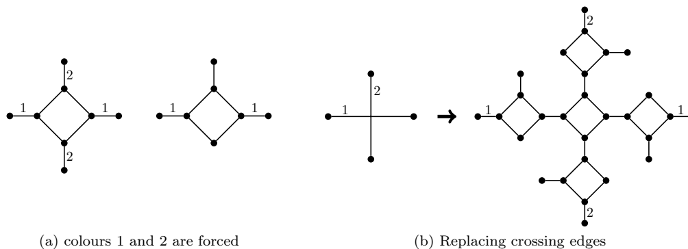
Figure 8: Transporting a colour in a strong 6-edge-colouring
