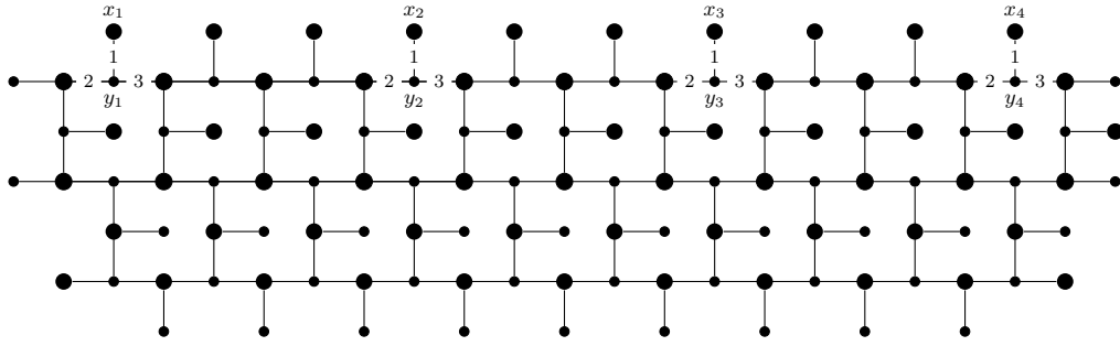
Figure 4: Vertex gadget for the case of girth 8 of Theorem 2
