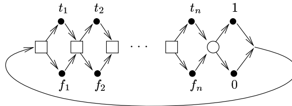
Figure 4. The arena of the game G(h, n)
