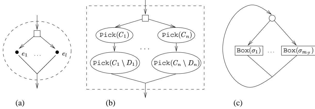
Figure 3. The arena \mathcal{A}_{\mathcal{F}} .
