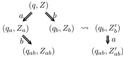
Figure 5: A diamond that is destroyed by a subsumption.
