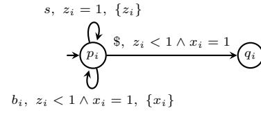
Figure 8: A process in our second example.
