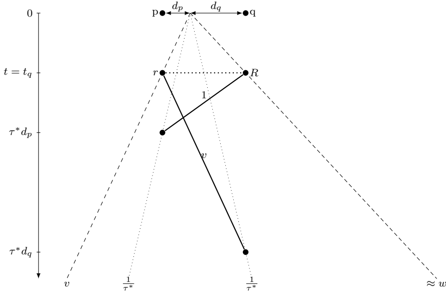
Fig. 7 Illustration of notions used in the first part of the proof of Lemma 4.6. The slower robot r , while discovering p at time t , must be able to reach q before \tau^* d_q . Similarly, the robot discovering q at time t_q must be able to reach p before \tau^* d_p .
