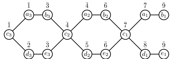
Figure 1: The initial configuration of G_3
