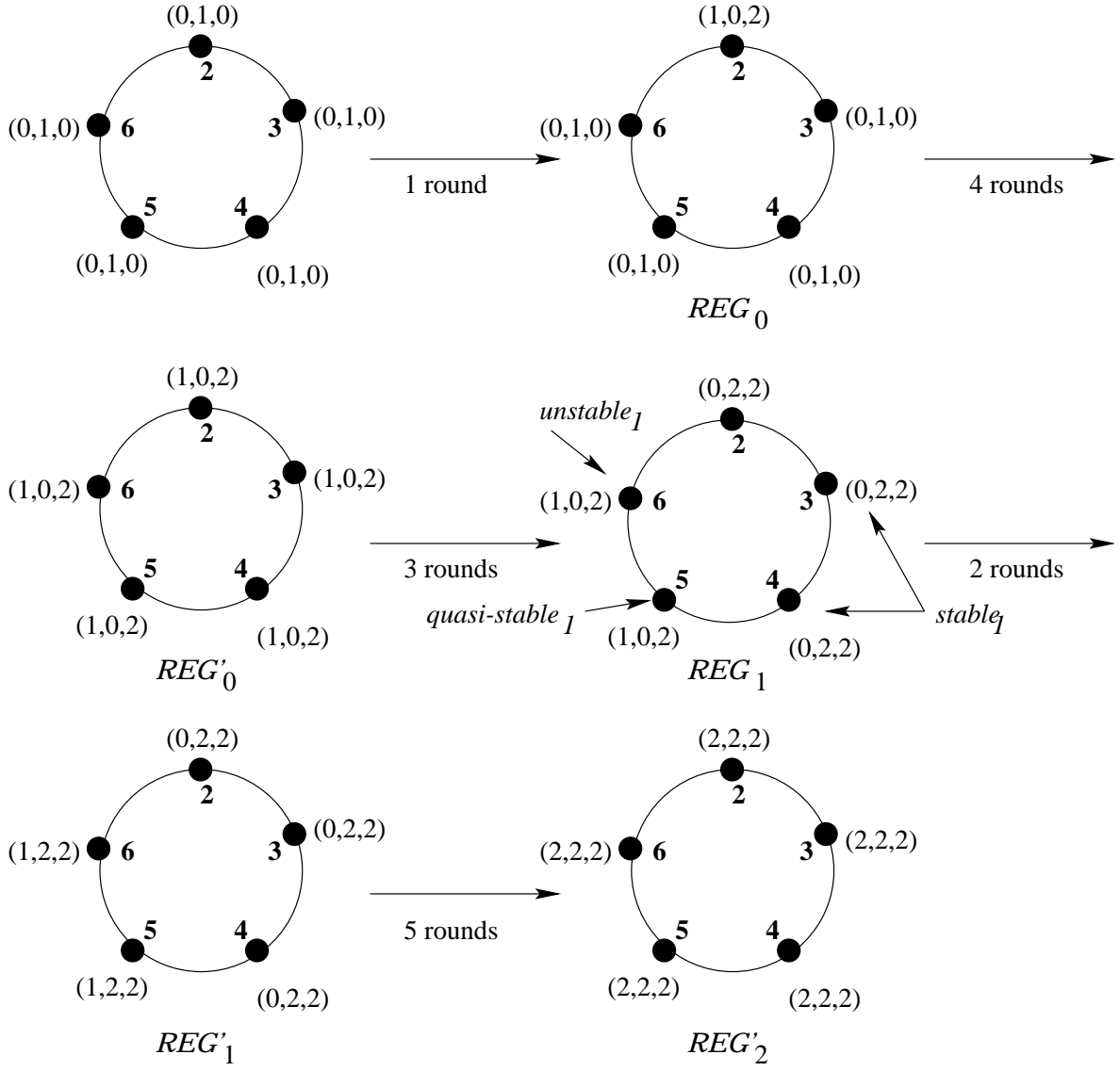
Figure 2: stabilization in a 5-Ring that is 1-bounded
