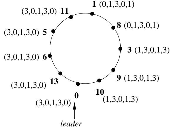
Figure 1: the deadlock configuration in a 10-Ring that is 3-bounded
