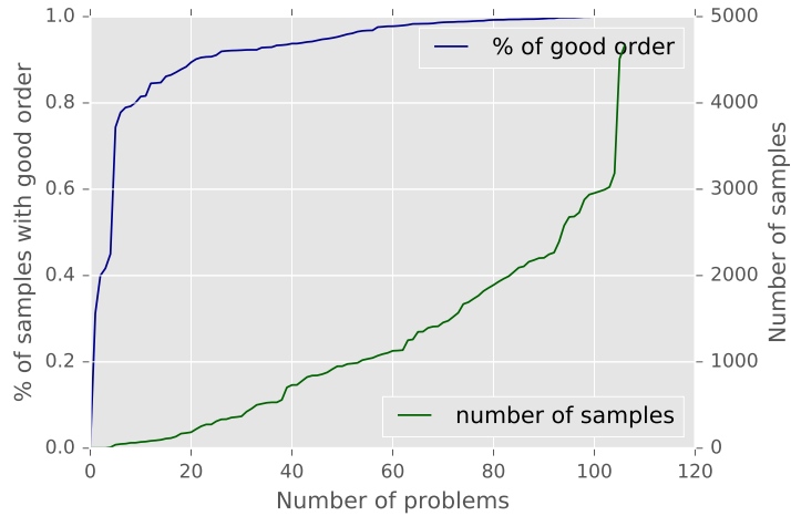
Fig. 5. CDF of the percentage of samples s.t. (max - min)_{dec} \leq (max - min)_{learnt} \leq (max - min)_{res} (left Y-axis). We also report the CDF of the number of samples per problem (right Y-axis).
