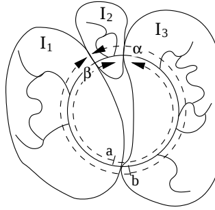
Figure 2: Split of the vertices set to handle cycles.
