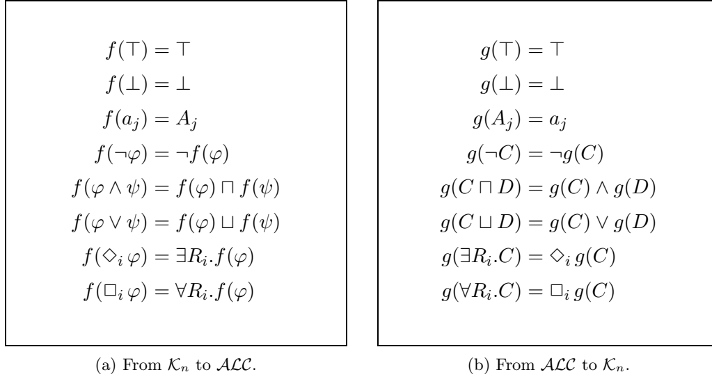
Figure 2.4: Mapping between \mathcal{K}_n formulae and \mathcal{ALC} concept expressions.
