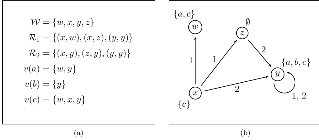
Figure 2.1: An example model and its graphical representation.
