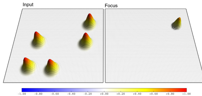
Fig. 1. The model of attention is made of two maps (input and focus), each of them being of size n \times n units ( n = 40 in experiments). Input map (on the left) corresponds to an entry that is feeding the focus map (on the right) which represents a cortical layer whose units possess localized receptive fields on the surface of the input. In other words, each unit x_{ij} of focus map receives its input from the input map which corresponds to a localized receptive field, being more or less broad depending on some constants. The input map does not have any lateral interaction or feed-back while each unit in the focus map is laterally connected using a difference of Gaussian. Activation of units from the focus map is governed by an equation introduced by Amari (1977) and extended by Taylor (1999) which considers a neural continuum governed by a simple differential equation. This architecture implements the most rudimentary form of attention that allows the model to focus on one static or moving stimulus without being disturbed by noise, movement or distractors.
