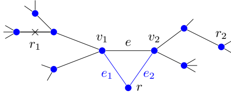
Figure 9: Construction of G^+ .
