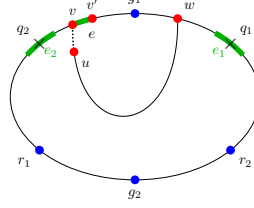
Figure 17: w is on Q[q_1, g_1] .
