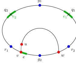
Figure 24: w is on Q[g_2, r_2] .
