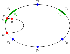
Figure 19: w is on Q[v, r_1]
