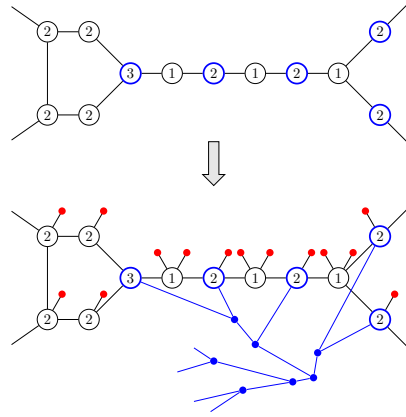
Figure 7: Construction of G from G' .
