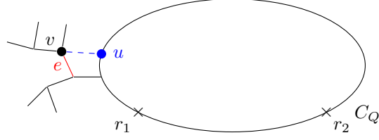
Figure 13: Case when v \notin V(C_Q) .
