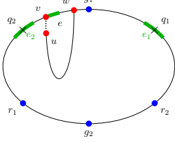
Figure 16: w is on Q[g_1, v] .
