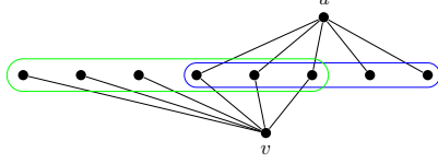
Figure 2: Case when uv \notin E(G) .
