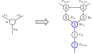
Figure 5: The gadget for an OR vertex.
