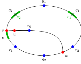
Figure 21: w is on Q[g_2, r_2]
