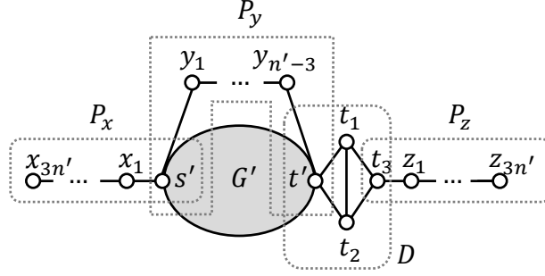
Figure 8: The graph G in the corresponding instance.
