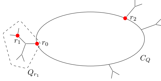
Figure 12: Case when r_1 \notin V(C_Q) and r_2 \notin V(Q_{r_1}) .
