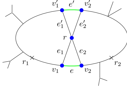
Figure 10: Construction of G^+ .
