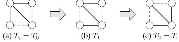
Figure 1: A reconfiguration sequence from T_s to T_t (with no constraint on spanning trees). There is no reconfiguration sequence from T_s to T_t if we restrict spanning trees either with maximum degree at least three or with diameter at most two.
