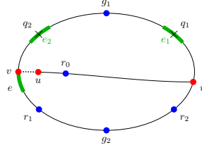
Figure 22: w is on Q[r_2, q_1]
