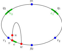
Figure 23: w is on Q[v, g_2] .
