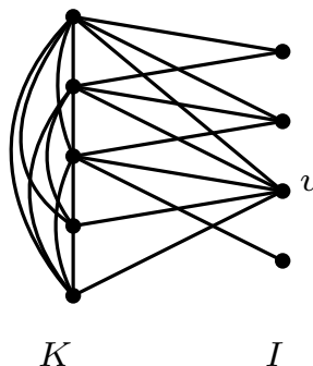
Figure 1.11 – Split graph G .
