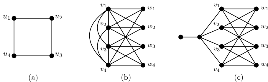
Figure 2.10 – (a) Original graph with (b) corresponding split graph and (c) bipartite graph.
