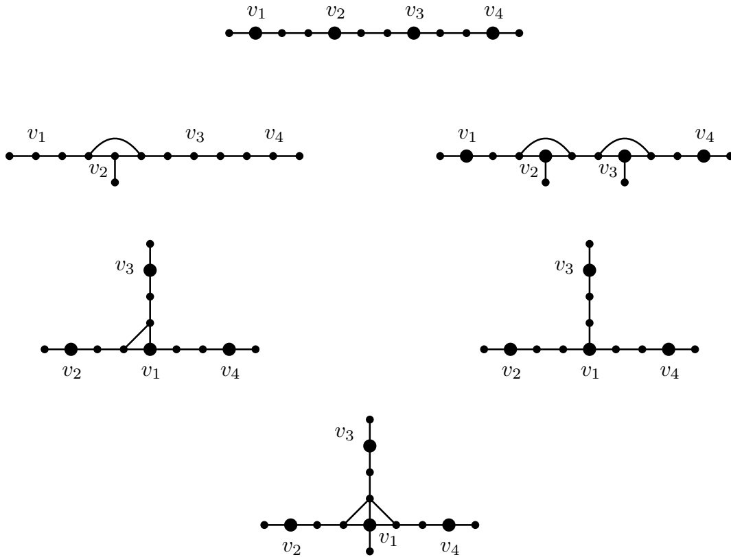
Figure 2.25 – Any graph from \mathcal{T}_4 is obtained from one of these graphs by adding a (non necessarily maximal) matching between the leaves.
