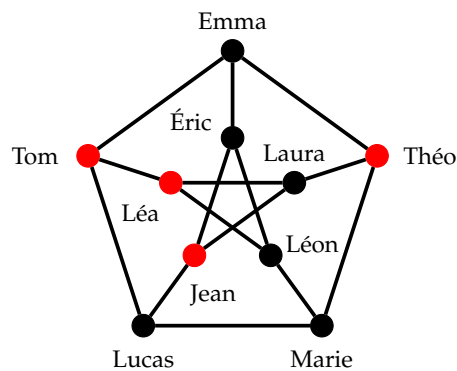
Figure 1.24 – Modeling of this problem: the dominating set is depicted by the red vertices.
