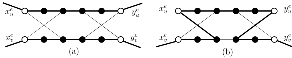
Figure 4.5 – The two possible subgraphs around a regular edge-gadget \mathcal{G} . Thick edges are edges in the tree. Edges with one endpoint in the gadget are edges of \delta(\mathcal{G}) .
