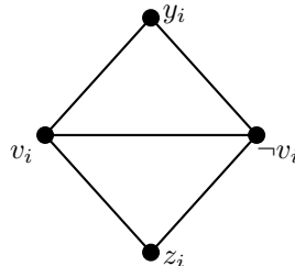
Figure 2.7 – The gadget \mathcal{G}_i corresponding to the variable x_i of \phi .
