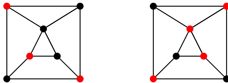
Figure 1.35 – A maximum independent set whose complement is a minimum vertex cover.
