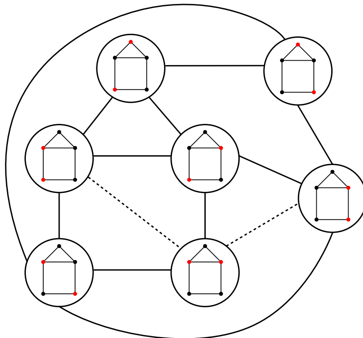
Figure 3.1 – \gamma -graph of the House graph under TJ (where we take into account the dashed edges). If we remove the dashed edges, it is the \gamma -graph under TS.
