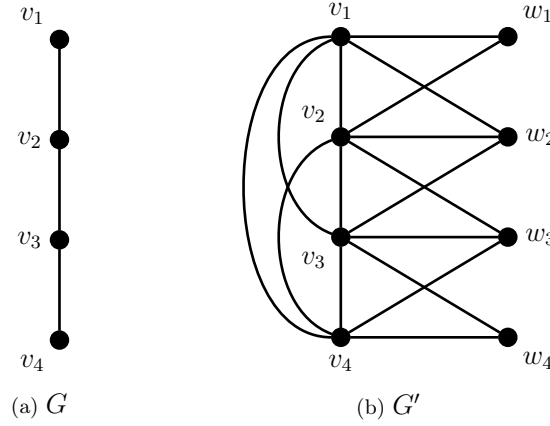
Figure 3.10 – Example for the reduction of Theorem 3.19.
