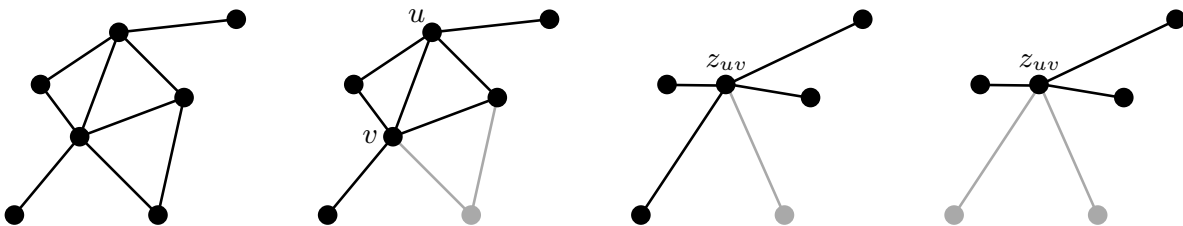
Figure 1.4 – The rightmost graph is a minor of the leftmost one. The third graph in this sequence is obtained from the second by contracting the edge uv .
