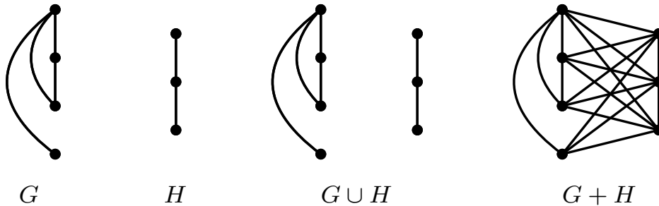
Figure 1.14 – Graphs G and H , and their disjoint union G \cup H and join G + H .
