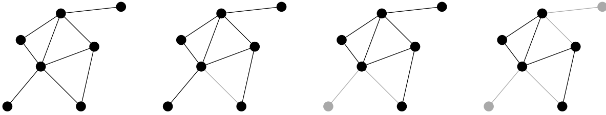
Figure 1.3 – Sequence of removals of vertices and edges: the rightmost graph is a subgraph of the leftmost one, but not an induced one.
