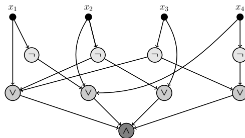
Figure 1.17 – Boolean circuit corresponding to the boolean formula \phi of Example 1.10.
