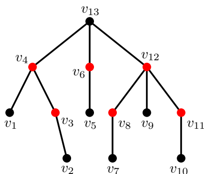
Figure 2.13 – Minimum dominating set \{v_3, v_4, v_6, v_8, v_{11}, v_{12}\} of a tree T .
