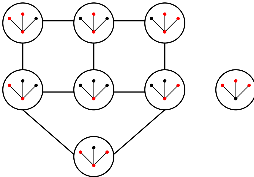
Figure 3.2 – The reconfiguration graph \mathcal{R}_3(K_{1,3}) is disconnected.
