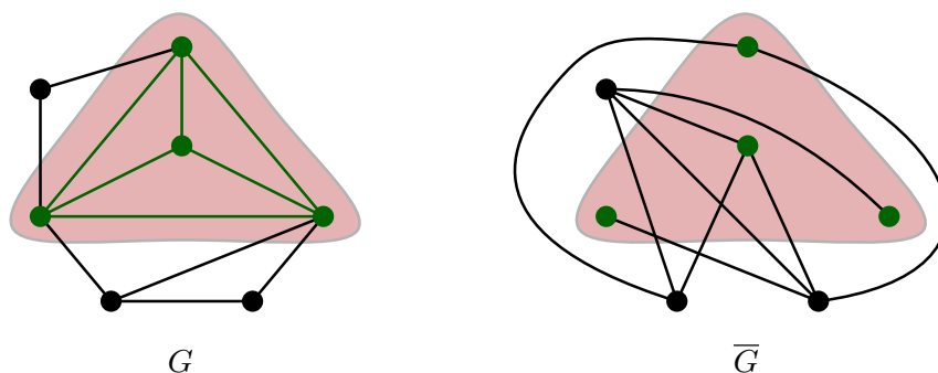
Figure 1.5 – Graph G and its complement \overline{G} . The graph induced by the green vertices is a clique of size four in G , and an independent set in \overline{G} .
