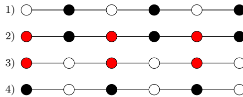
Figure 4.13 – In the input graph, a bipartition is given. Therefore, the target coloring can be reached by using one extra color in three steps.
