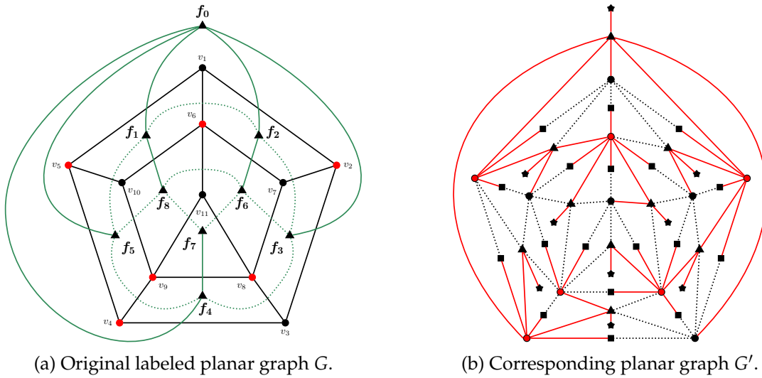
Figure 4.2 – Reduction for Theorem 4.3. The vertex cover C of G is depicted by the red vertices. The dual graph is the graph induced by the green edges. The spanning tree obtained by the BFS is represented by the solid edges. The face-vertices (respectively edge-vertices) of G' are depicted by triangles (resp. squares). The spanning tree T of G' associated with the vertex cover C is the tree induced by the red edges. The number of leaves of T is 2(|E(G)| + 1) - |C| = 32 .
