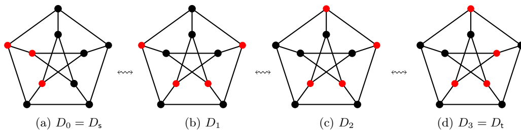
Figure 4 – Reconfiguration sequence between two dominating sets of the Petersen graph.
