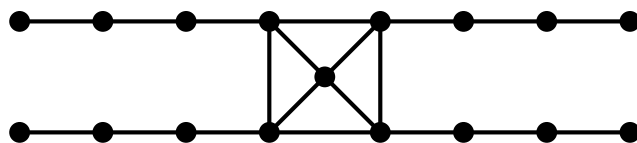
Figure 2.26 – Counterexample for Conjecture 2.44.
