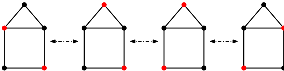
Figure 1.33 – Reconfiguration sequence of independent sets with rule (ii).
