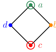
(a) Original instance (G, k) of MINIMUM VERTEX COVER with a vertex cover \{a, c\} .
