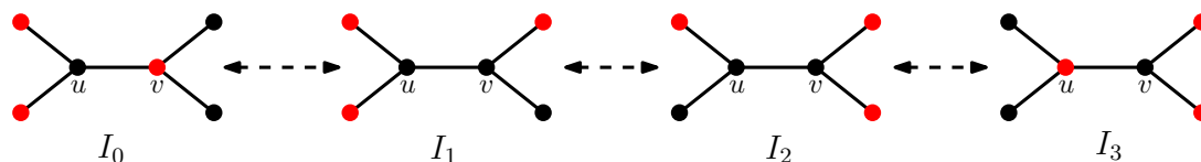
Figure 1.36 – Reconfiguration sequence under TJ between two independent sets I_0 and I_3 .
