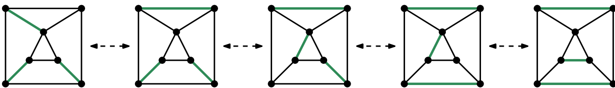
Figure 1.31 – Reconfiguration sequence of perfect matchings via edge flips.
