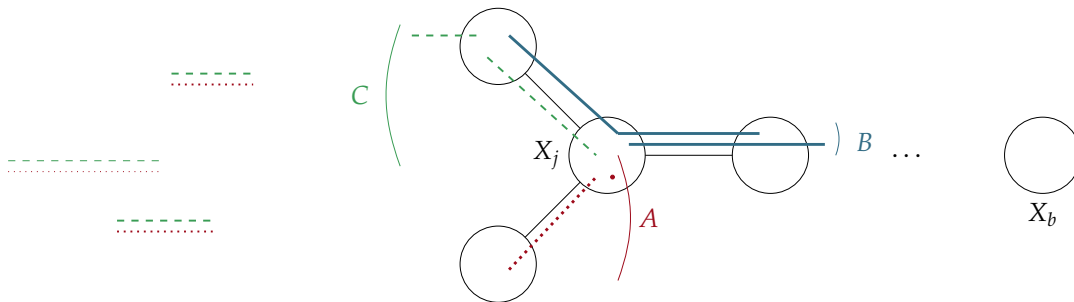
Figure 3.4 – The tree decomposition of G , and the sets A , B and C . The circles represent the bags of the tree decomposition. The vertices are represented by lines, or dots, that go throughout the bags they belong to. The thick full lines represent the vertices of B , the dashed lines represent the vertices of D , and the dotted lines represent the vertices of D_j . By the induction hypothesis, the left vertices of D_j that do not belong to X_j belong to D .
