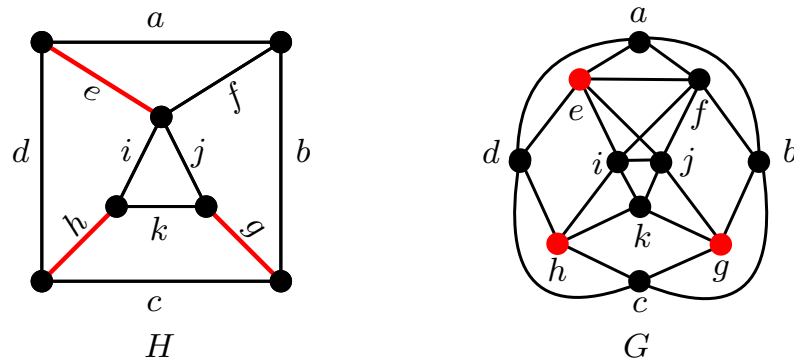
Figure 1.34 – Maximum matching in H and the corresponding maximum independent set in its line graph G .
