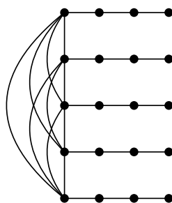
Figure 2.16 – The graph G_5 .
