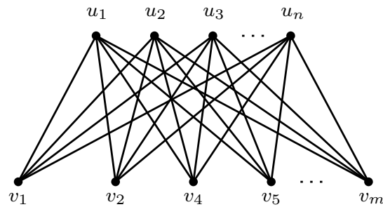
Figure 1.9 – Complete bipartite graph K_{n,m} .
