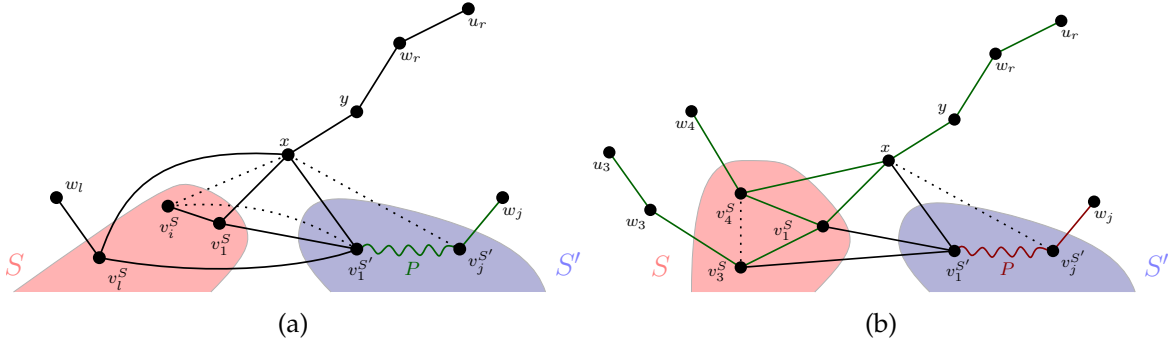
Figure 2.19 – Illustration for the proof of Case 1 of Lemma 2.41
