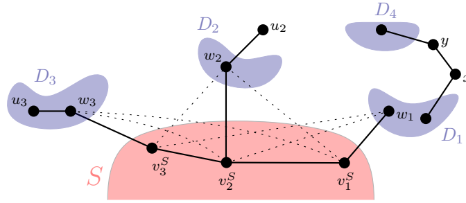
Figure 2.18 – The vertex x is 4-linking for S .
