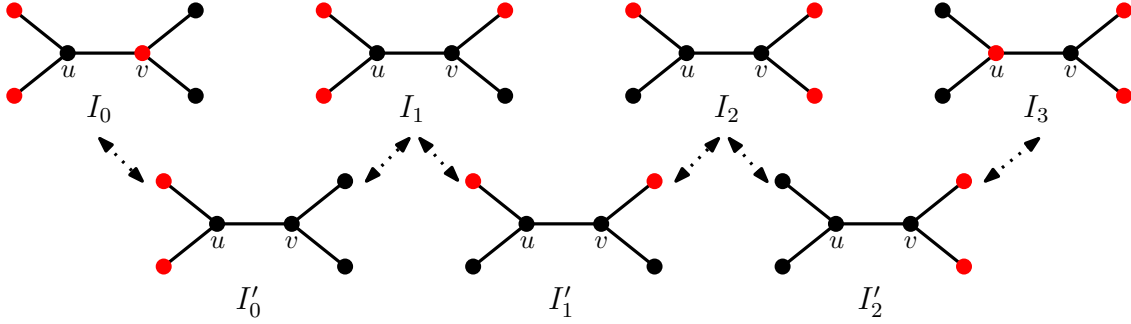
Figure 1.37 – Reconfiguration sequence under TAR between two independent sets I_0 and I_3 .
