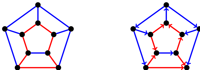
Figure 1.28 – A possible instance for the NCL problem and a feasible solution for this instance.
