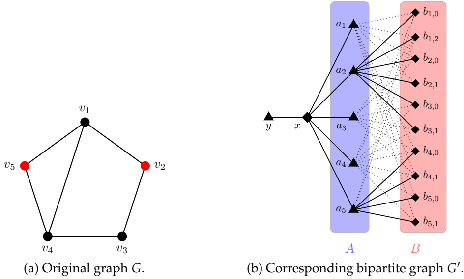
Figure 4.1 – Example for the reduction of Theorem 4.2: the dominating set D = \{v_2, v_5\} of G is depicted by the red vertices and the spanning tree of G' associated with D is the tree induced by the solid edges. For the split case, we add all the possible edges in G'[A] so that G'[A \cup \{x\}] is a clique and G'[B \cup \{y\}] an independent set.
