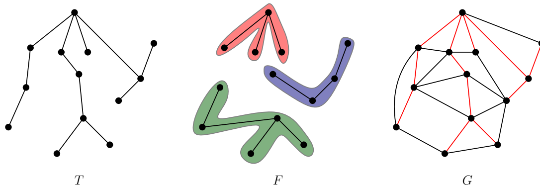
Figure 1.7 – A tree T and a forest F with three connected components, each of them being a tree. The red edges of the graph G induce a spanning tree of G .
