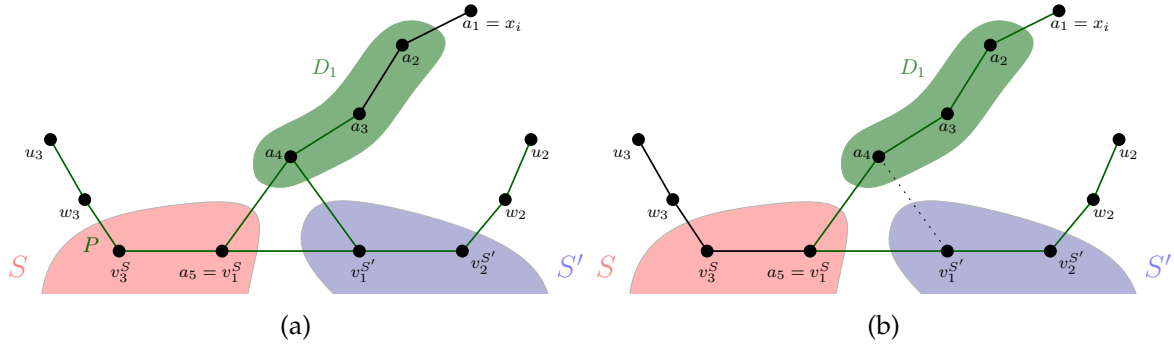
Figure 2.23 – Illustration for the proof of Claim 1 where |P| \geq 5 .
