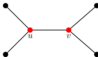
Figure 2.5 – The set \{u, v\} is a minimal dominating set, but not a stable set.
