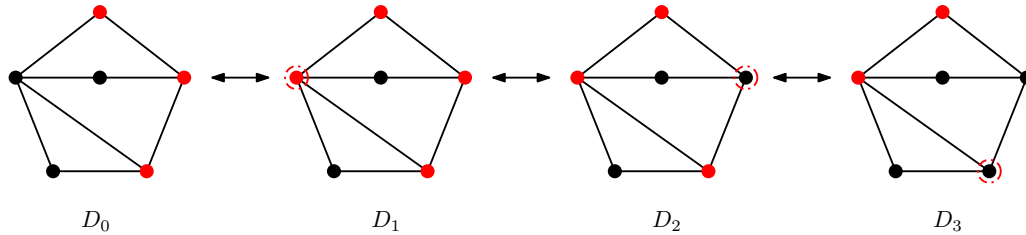
Figure 3.16 – Reconfiguration sequence between D_0 and D_3 via dominating sets D_1, D_2 with upper bound k = 4 , where added or removed vertices are surrounded by dotted circles.
