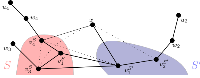
Figure 2.21 – Case 3 of Lemma 2.41: q = 4 .
