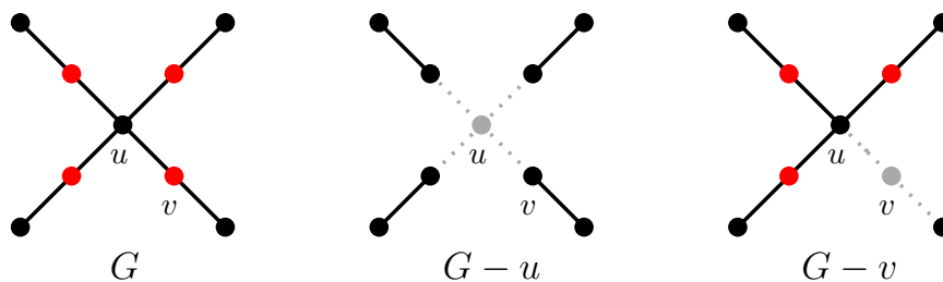
Figure 1.16 – G has a vertex cover of size four depicted by the red vertices but G - u has no vertex cover of size three. However, G - v has a vertex cover of size three.
