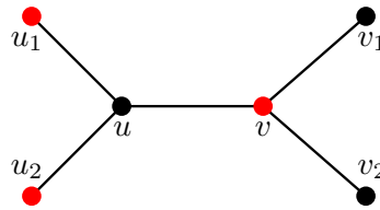
Figure 2.6 – The set \{u_1, u_2, v\} is a maximal independent set.
