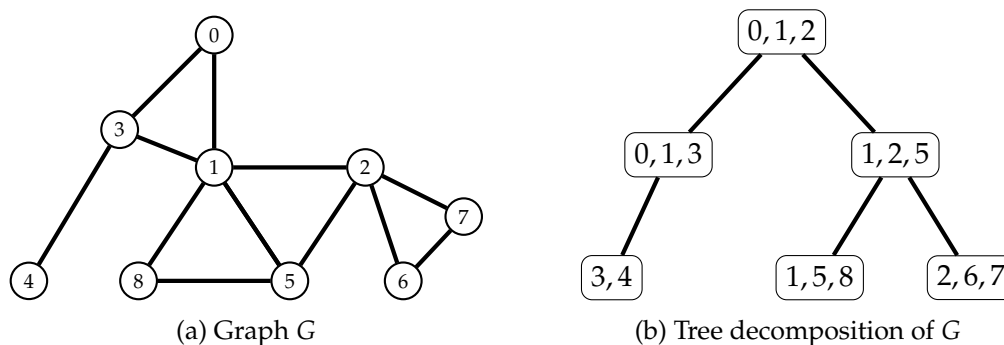
Figure 1.20 – Graph G and a tree decomposition of G of width two.
