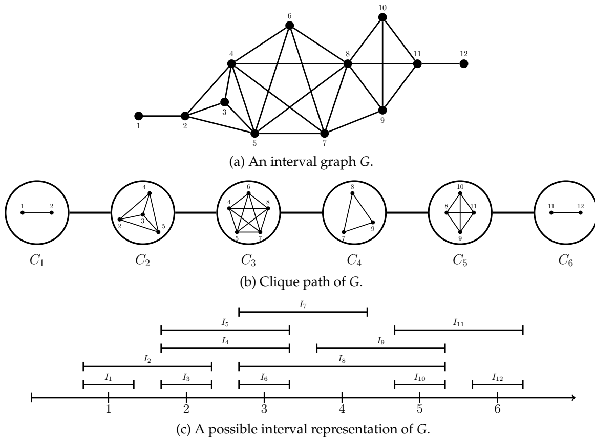
Figure 1.12 – Interval graph and an interval representation obtained from the clique path of G .
