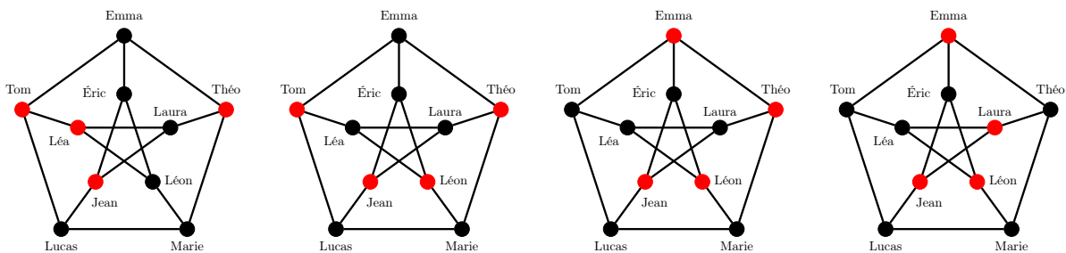
Figure 1.25 – Modification of the committee \{\text{Jean, Léa, Théo, Tom}\} into the committee \{\text{Emma, Léon, Jean, Laura}\} , where each intermediate committee is a valid one.
