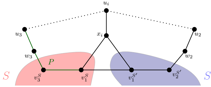
Figure 2.24 – Illustration for the proof of Lemma 2.42: the only possible missing edges are the dotted ones.
