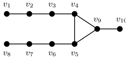
Figure 1 – The third forbidden induced subgraph.
