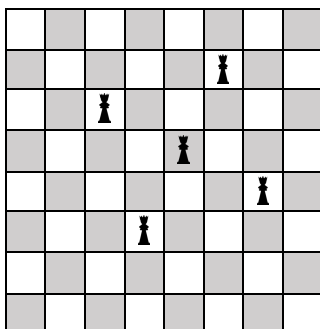
Figure 2.2 – A possible solution.
