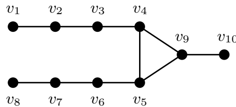
Figure 2.17 – The graph H .
