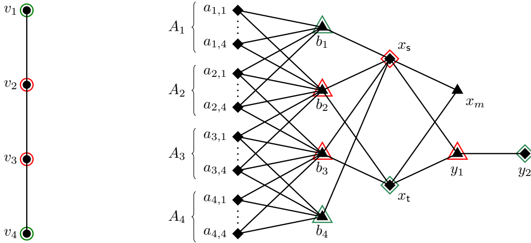
Figure 3.22 – Example for the reduction of Theorem 3.50: the original instance is (G, D_s = \{v_2, v_3\}, D_t = \{v_1, v_4\}) and the corresponding instance (G', 5, 4, D'_s = \{b_2, b_3, x_s, y_1\}) of OPT-IDSR, where G' is a bipartite graph. The only independent dominating set of size k + 2 = 4 of G' is D_t = \{b_1, b_4, x_t, y_2\} .
