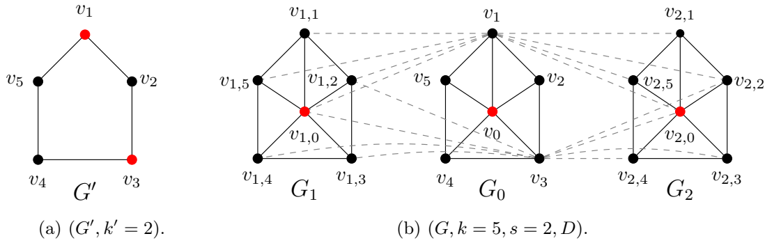
Figure 3.20 – Reduction for Theorem 3.40 with D' = \{v_1, v_3\} and D = \{v_0, v_{1,0}, v_{2,0}\} .
