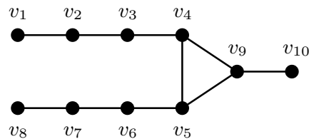
Figure 5 – The third forbidden induced subgraph.
