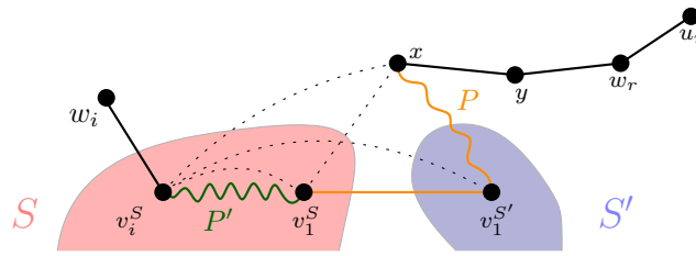
Figure 2.20 – Illustration for the proof of Case 2.
