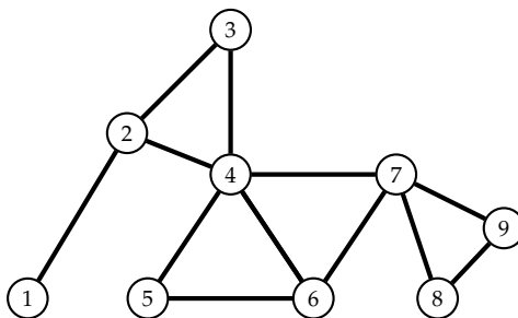
Figure 1.22 – Labeling of a graph G of bandwidth at most three.
