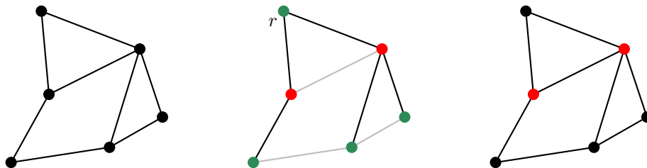
Figure 2.3 – Illustration for the proof of Proposition 2.1: the red vertices dominate the graph.
