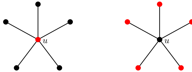
Figure 2.4 – A minimum dominating set and an upper dominating set of K_{1,5} .
