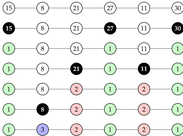
Figure 4.10 – Execution of the algorithm on a P_6 .
