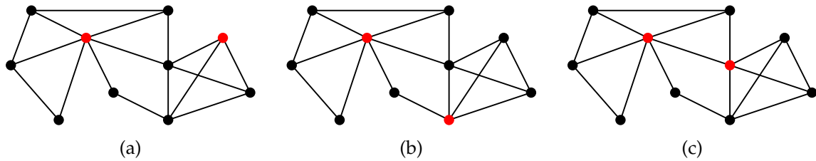
Figure 3 – Three different dominating sets of size two of the same graph.
