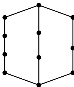
Figure 4.14 – A theta graph.
