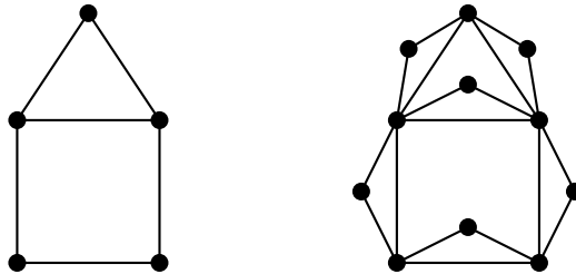
Figure 2.9 – Reduction from VERTEX COVER to DOMINATING SET.
