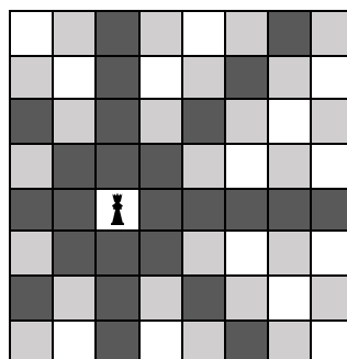
Figure 2.1 – The queen can move to any dark gray shaded square.
