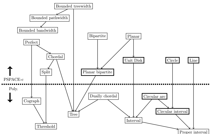
Figure 3.15 – Complexity of \text{DSR}_{T5} with the results by Bousquet and Joffard [Jof20].
