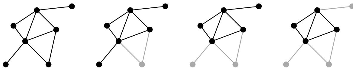
Figure 1.2 – The rightmost graph is an induced subgraph of the leftmost one.
