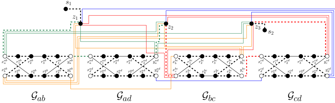
(b) Graph H(G) obtained from the reduction. The ordering for the vertices of the vertex cover \{a, c\} of G is the lexicographic order, as well as the ordering of the edges incident to each vertex. The corresponding Hamiltonian path is depicted by the thick dashed edges.
