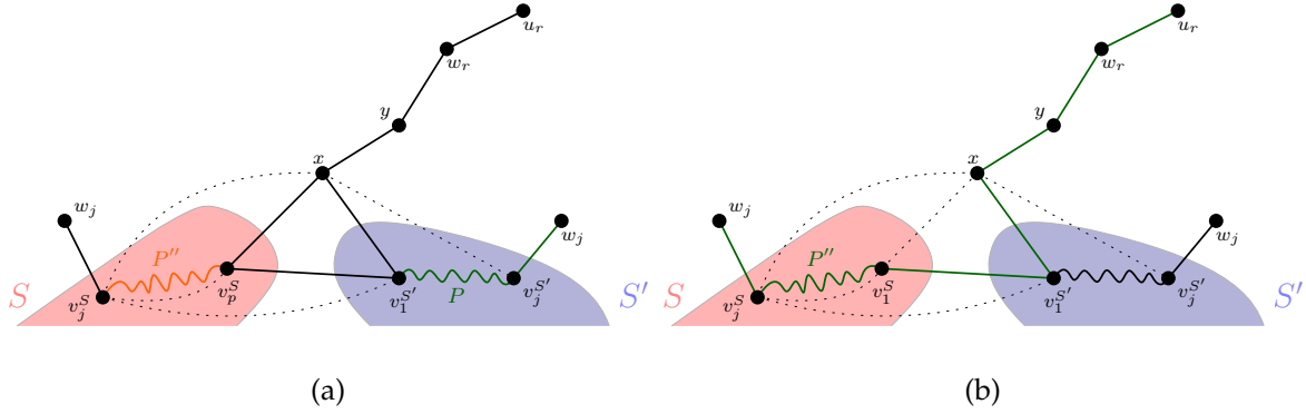
Figure 2.22 – Illustration for the proof of Case 3 of Lemma 2.41.
