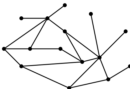
Figure 1.13 – A planar graph with a planar drawing.
