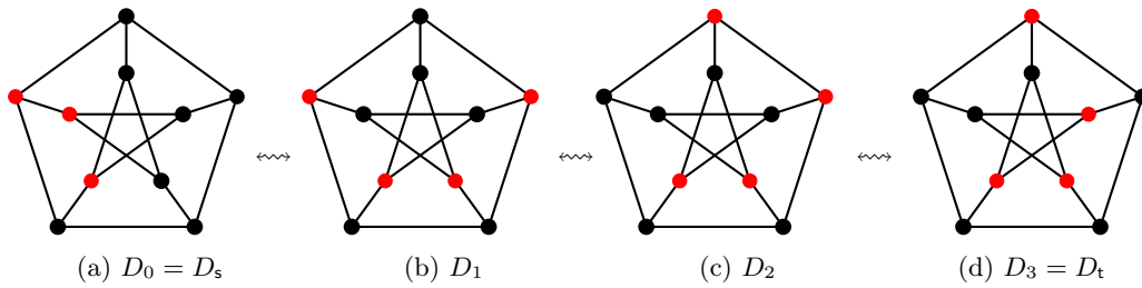
Figure 3.8 – Example of TS-sequence from D_s to D_t .
