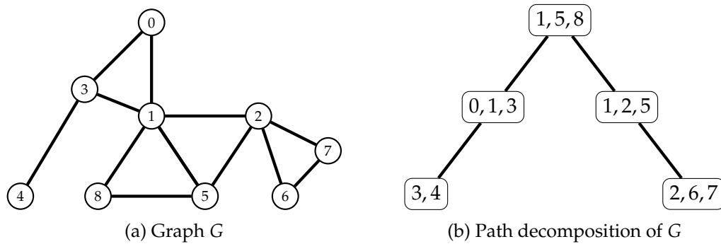
Figure 1.21 – Path decomposition of the graph G seen in Figure 1.20a of width two.
