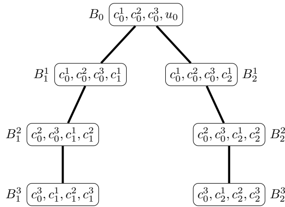
Figure 3.7 – Tree decomposition of G_{3,2} of width tw(G_{3,2}) .
