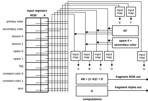
Figure 25: The final combiner stage is used to compute the resulting fragment output for RGB and Alpha.
