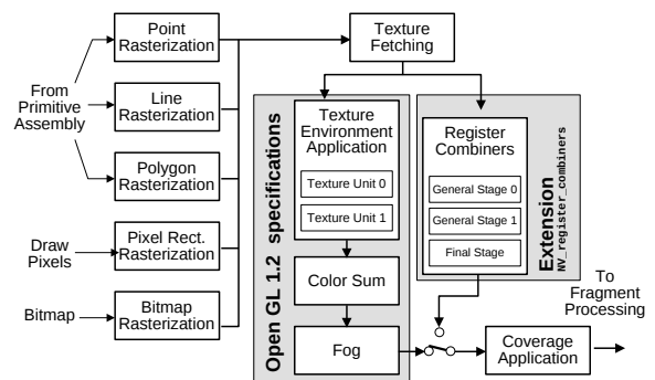
Figure 23: Since the multi-texture model of OpenGL 1.2 turns out to be too limiting, NVidia's GeForce 256 processor provides multi-stage register combiners that completely bypass the standard texturing unit.
