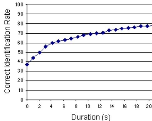
Figure 2 - Correct Identification rate in function of duration of test excerpts (Rhythm Model).
