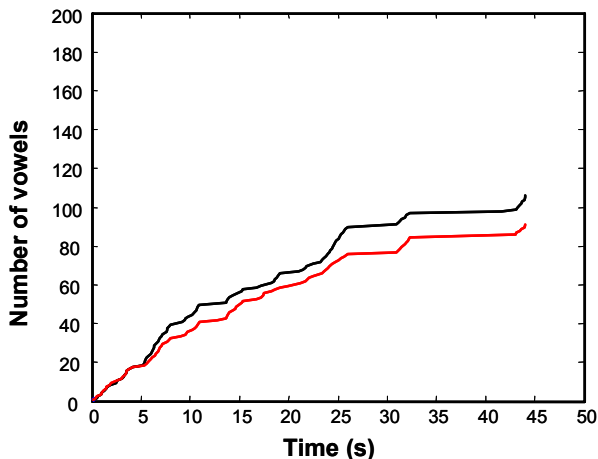
Figure 1: Example of the evolution of the number of vowels per second (black line: hand labeled; red line: detected) for a German speaker (call145).
