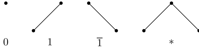
Figure 1.1: Game trees of games born by day 1.
