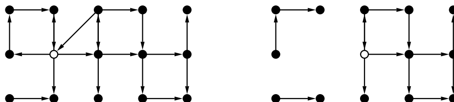
Figure 4.1: Playing a move in VERTEX GEOGRAPHY
