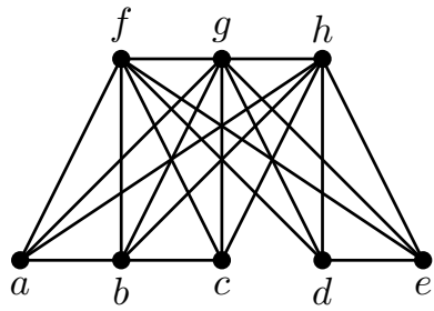
Figure 1.14: A cograph
