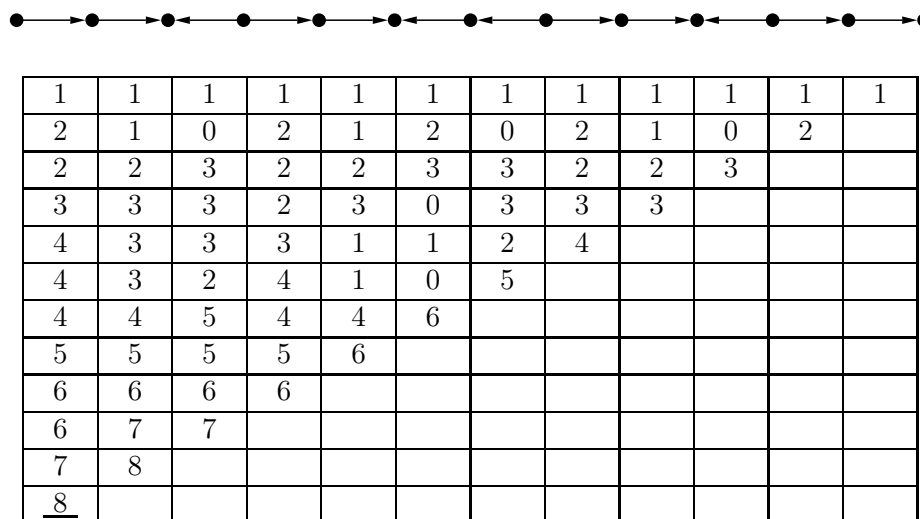
Figure 2.19: Computing the Grundy-value of a path
