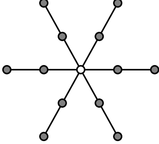
Figure 4.6: The tree Si_6^W
