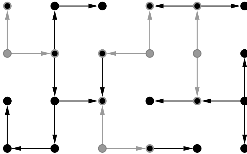
Figure 2.15: An orientation of a tree seen as a TIMBER position
