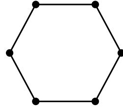
Figure 1.6: The cycle on six vertices
