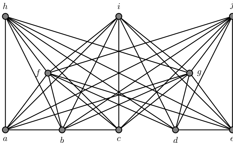
Figure 3.20: A cograph
