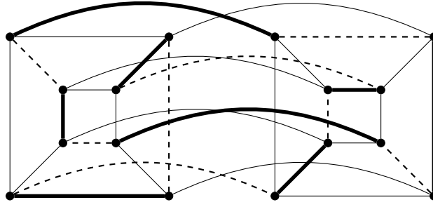
Figure 4.5: Two disjoint edge-identifying codes of \mathcal{H}_4 .
