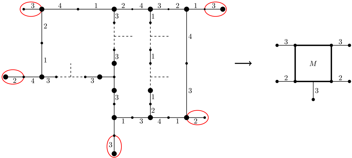
Figure 3.23: Sub-gadget M
