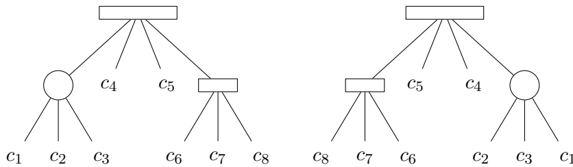
Figure 2.5: Equivalent PQ-trees
