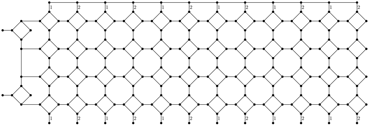
Figure 3.32: Graph P and some of its forced colours
