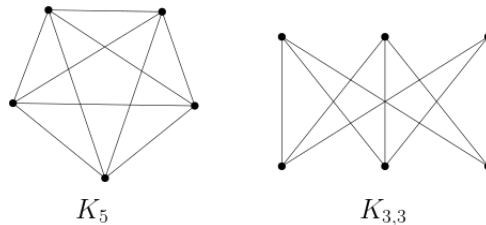
Figure 1.12: The two graphs whose subdivisions are obstruction to planarity.
