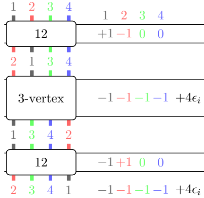
Figure 4.14: The evolution of a lollipop of a vertex v of degree 3 remains invariant even when a swap line the starting point u from v : first, two colors are swapped, then all the colors are rotated, 4\epsilon_i (with i being the color missing at the v ) compensating the rotation, and finally the swapped colors are swapped back.
