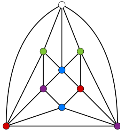
Figure 1.19: The Fritzsche graph with a partial coloring such that it is not possible to free a color for the white vertex using a single Kempe swap: a counter example to Kempe’s proof.
