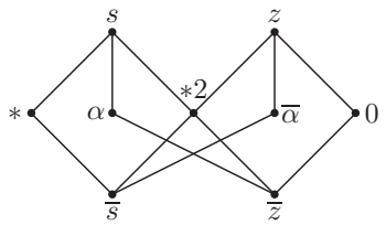
Figure 4: Partial ordering of dicots born by day 2
