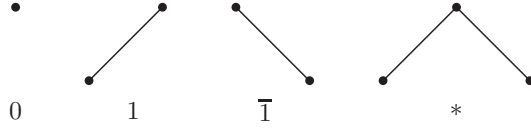
Figure 1: Game trees of games born by day 1.
