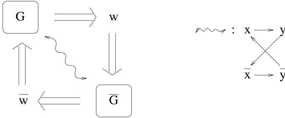
Figure 3: Tromp's construction
