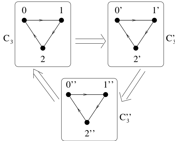
Figure 1: The graph C_3 \otimes C_3
