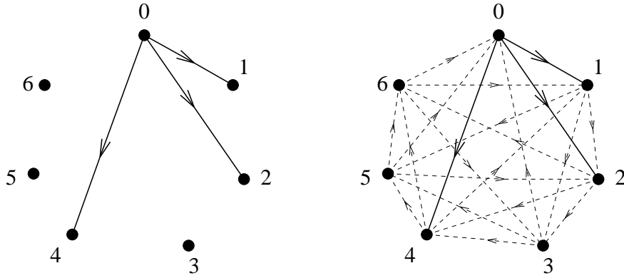
Figure 2: The tournament obtained from the quadratic residues of 7
