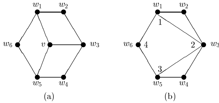
Figure 3: Configurations for Lemma 5
