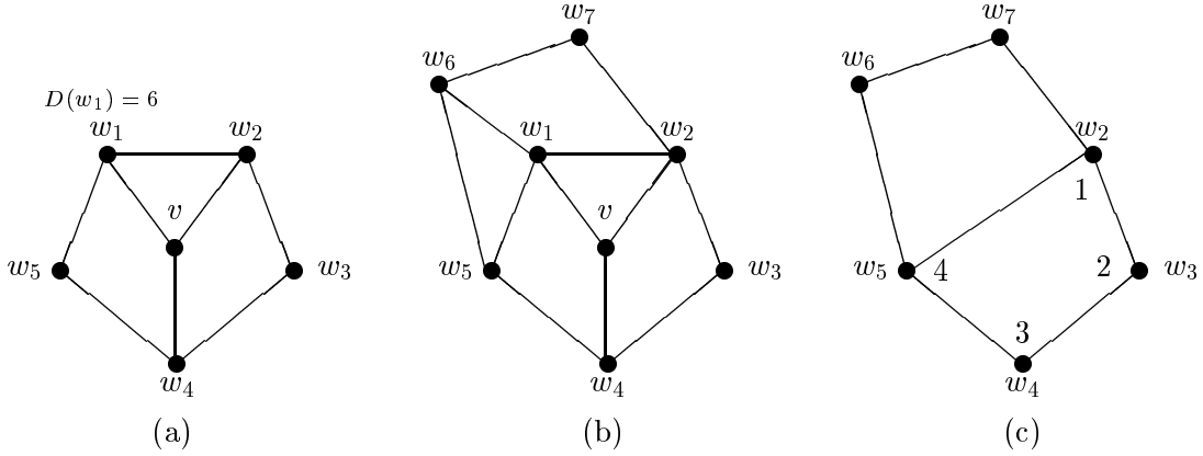
Figure 6: Configurations for Lemma 8
