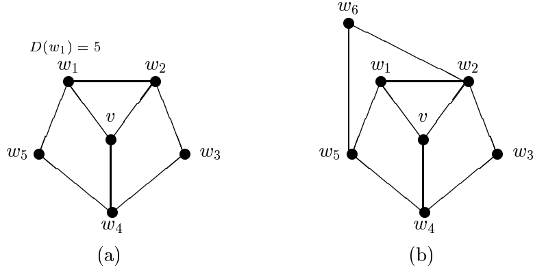
Figure 5: Configurations for Lemma 7
