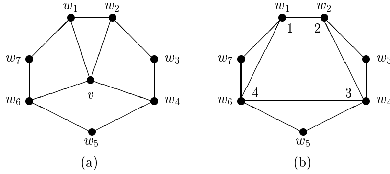
Figure 4: Configurations for Lemma 6
