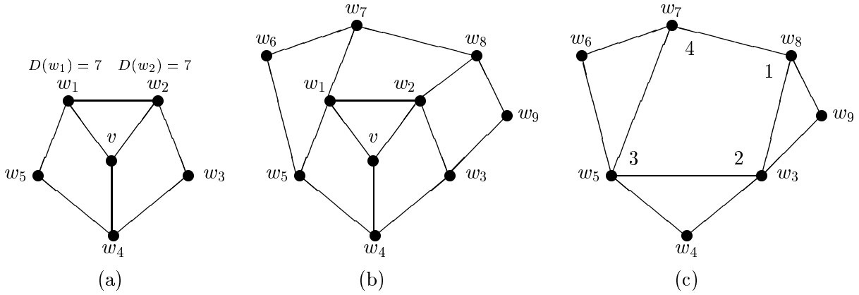
Figure 7: Configurations for Lemma 10
