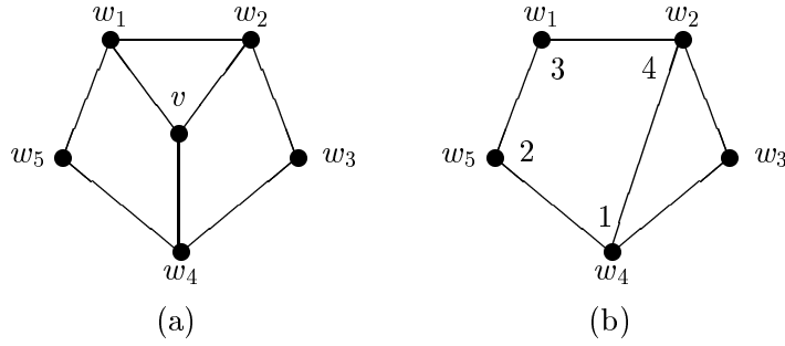
Figure 1: Configurations for Lemma 3
