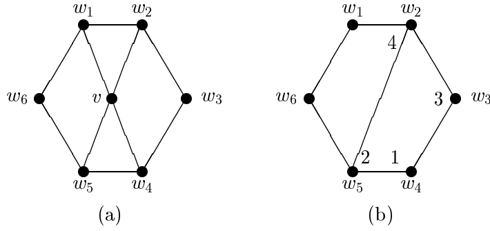
Figure 2: Configurations for Lemma 4
