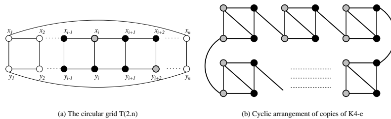
Figure 1: Negative results for graphs with maximum degree three
