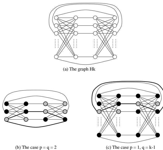
Figure 4: Construction for statement 2 of Theorem 6
