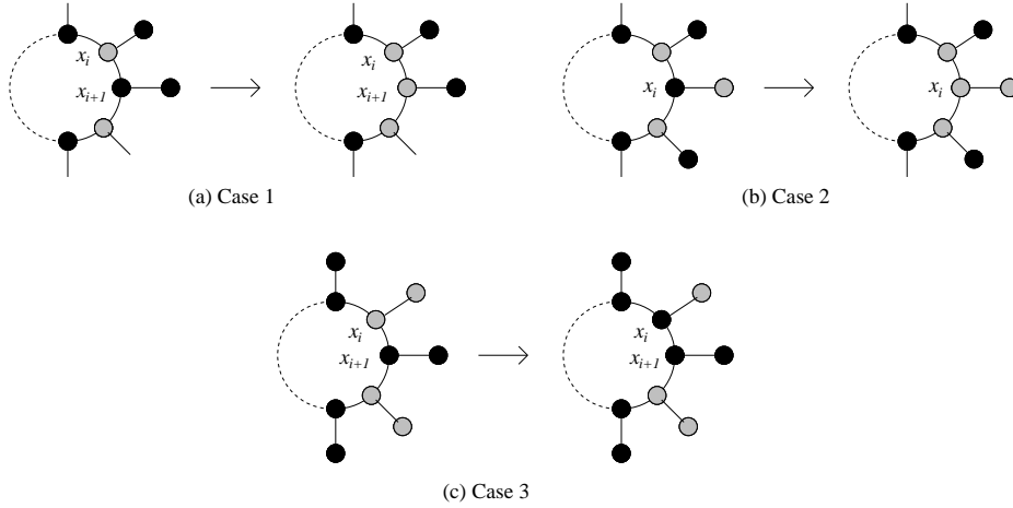
Figure 3: Deleting an alternating bichromatic cycle in a (\mathcal{T}_1, \mathcal{D}_2) -colouring
