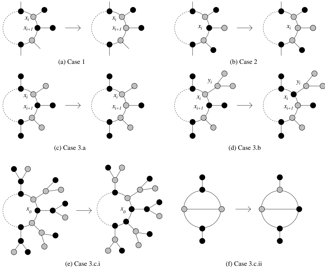
Figure 2: Deleting an alternating bichromatic cycle in a (\mathcal{T}_1, \mathcal{T}_1) -colouring
