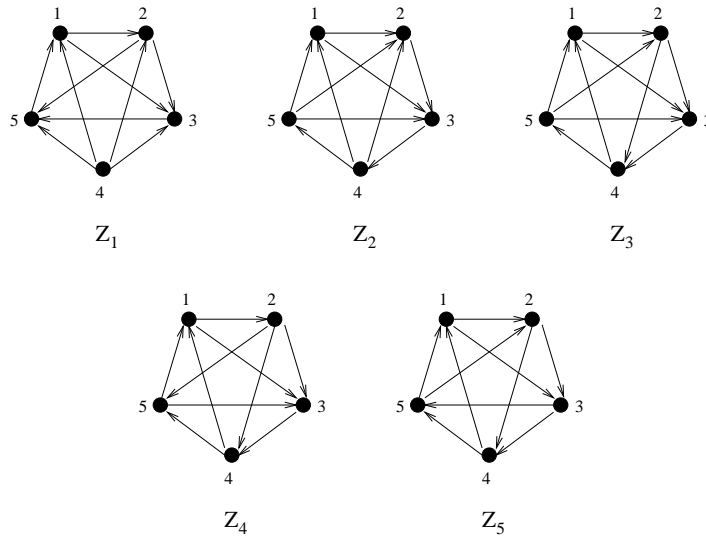
Figure 3: Target tournaments on five vertices
