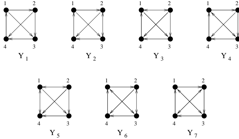
Figure 2: Target digraphs on four vertices
