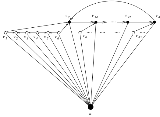
Figure 4: Construction of G_{Z_5,7}
