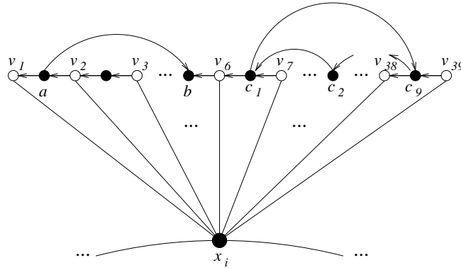
Figure 5: Construction of G_{X_5,8}
