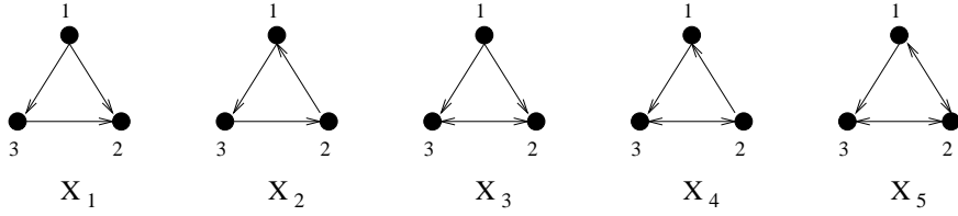
Figure 1: Target digraphs on three vertices
