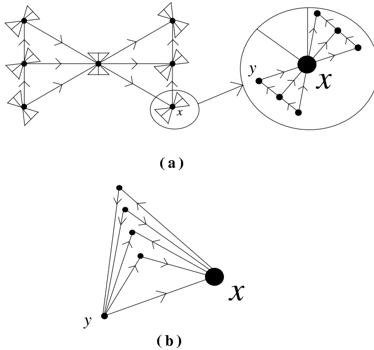
Figure 3: Construction of an oriented 3-tree with chromatic number 16
