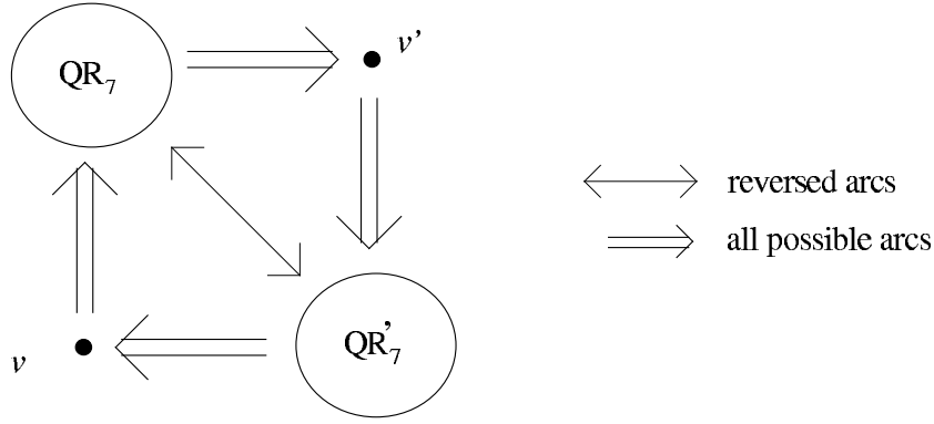
Figure 2: Tromp's construction
