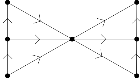
Figure 1: An oriented graph with chromatic number 7
