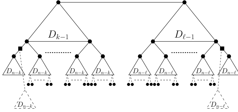
Figure 7: D_n^{k,\ell} is a subtree of \hat{D}_{n+1} (dashed lines depict elements of \hat{D}_{n+1} \setminus D_n^{k,\ell} )
