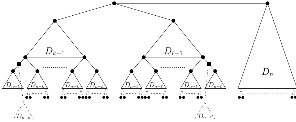
Figure 8: E_n^{k,\ell} is a subtree of \hat{D}_{n+1} (dashed lines depict elements of \hat{D}_{n+1} \setminus E_n^{k,\ell} )
