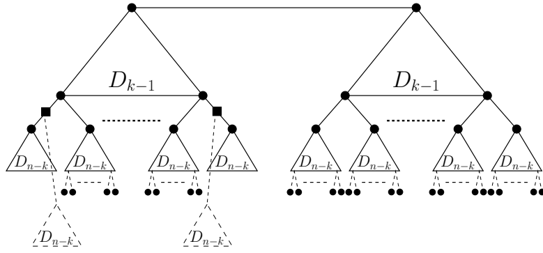
Figure 5: C_n^k is a subtree of \hat{D}_{n+1} (dashed lines depict elements of \hat{D}_{n+1} \setminus C_n^k )
