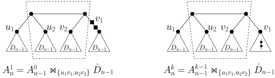
Figure 3: Structural decomposition of A_n^1 and of A_n^k , k > 1
