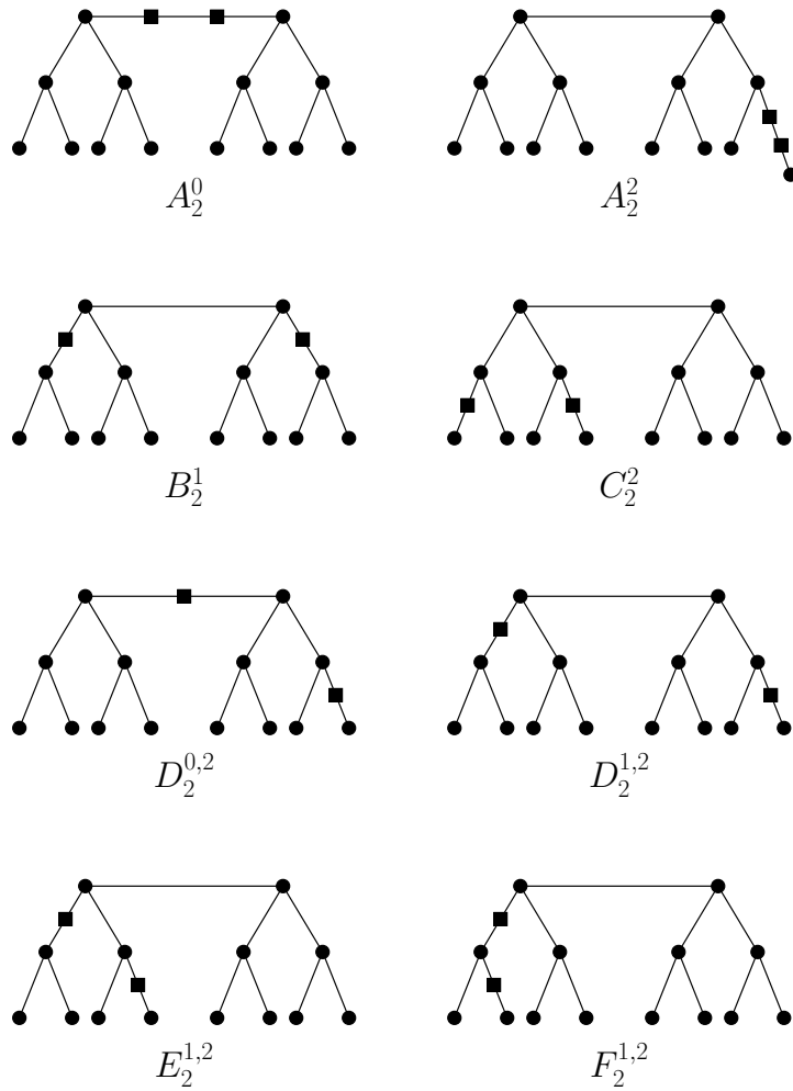
Figure 1: Sample twice subdivided 2-rooted complete binary trees
