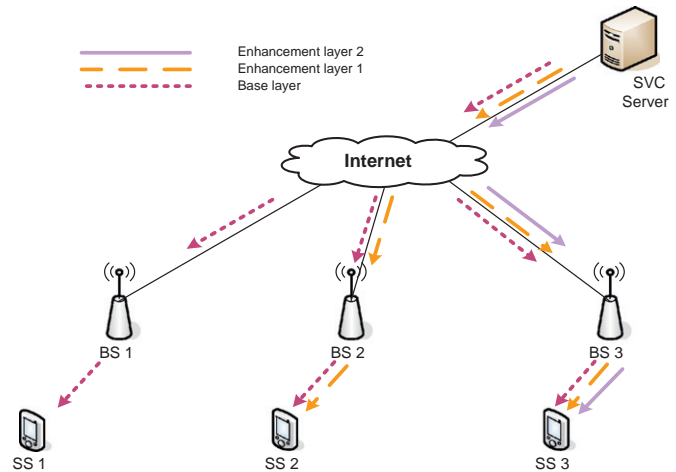
Fig. 9. Multi-cell architecture (multi-BS).
