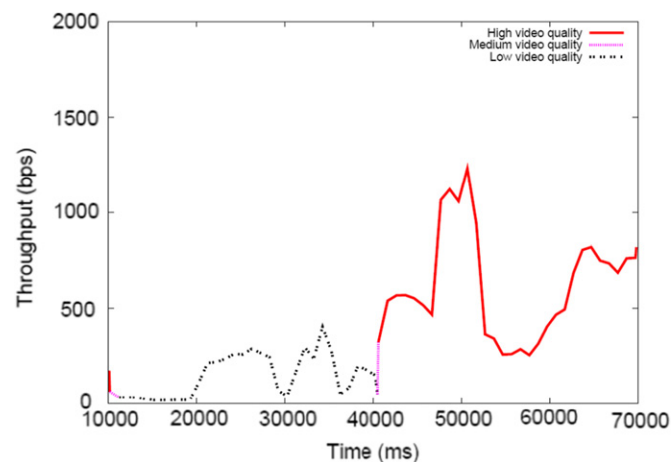
Fig. 17. Low quality increased to high quality video data rate during transmission.
