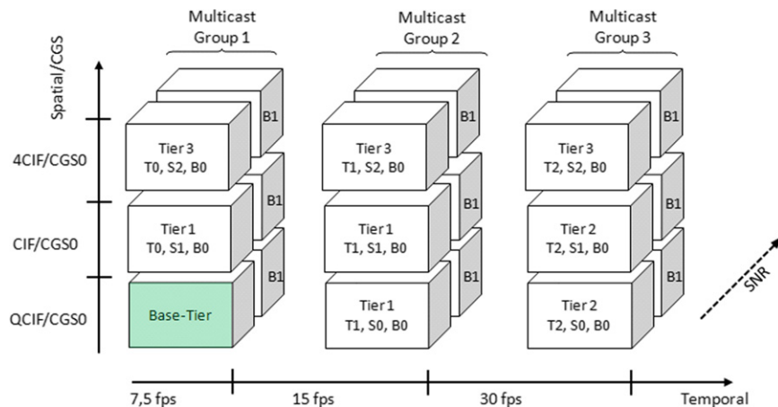
Fig. 8. Multicast group creation with SVC coding.
