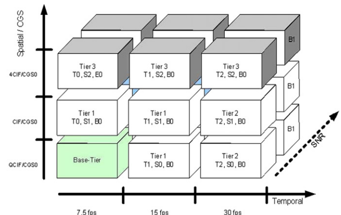
Fig. 2. SVC hierarchical level.
