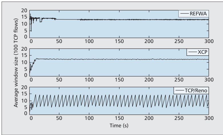
Figure 2. The average window size for REFWA, TCP, and XCP.
