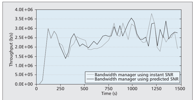
Figure 5. Throughput using instantaneous vs. predicted SNR.
