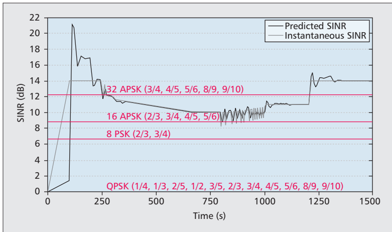
Figure 4. The instantaneous SNR vs. the predicted SNR.
