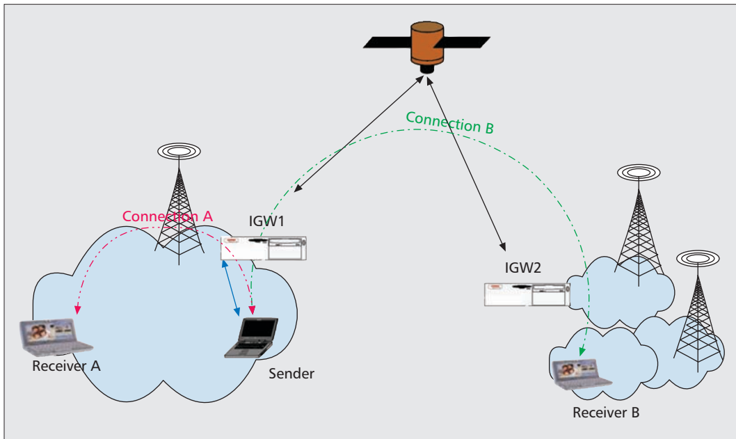
Figure 1. RTT-based connection setup + connection decoupling.
