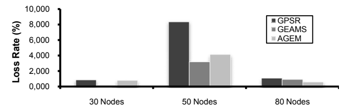
Figure 20 Packet-loss ratio in plain topologies.
