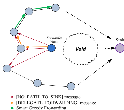
Figure 10 A blocking situation where a forwarder node has no neighbor closer to the sink node than itself.
