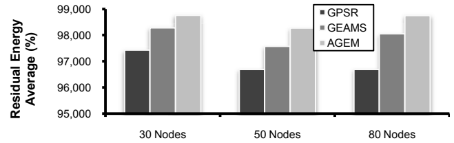
Figure 15 Average residual energy in “plain” topologies
