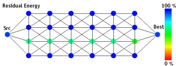
Figure 26 Residual energy with AGEM in a grid topology.
