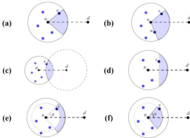
Figure 2 Greedy forwarding strategies: (a) Compass routing; (b) Random Compass routing; (c) Greedy routing; (d) Most Forwarding; (e) Nearest Neighbor routing; (f) Furthest Neighbor routing.
