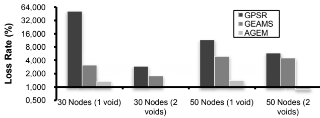
Figure 24 The packet-loss ratio in topologies with holes (please note the logarithmic scale)
