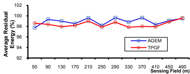
Figure 18 The distribution of the residual energy across the network for 80 nodes topology.
