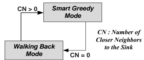
Figure 3 GEAMS Routing mode switching.
