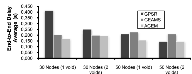
Figure 23 Average end-to-end delay in topologies with holes.
